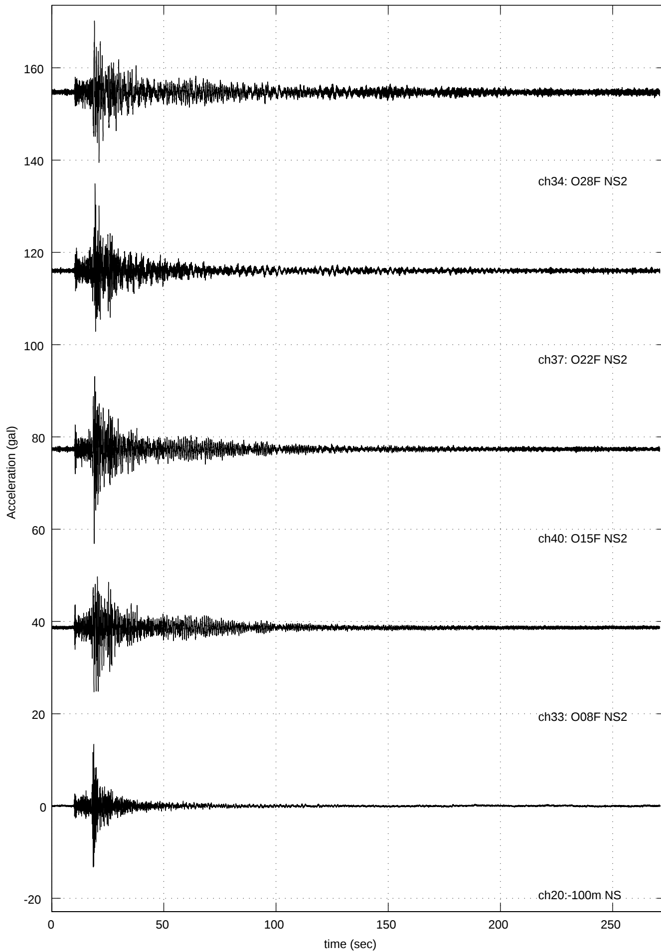
980829 Quake (O28F NS2: Max =15.47 at 19.1 sec )
