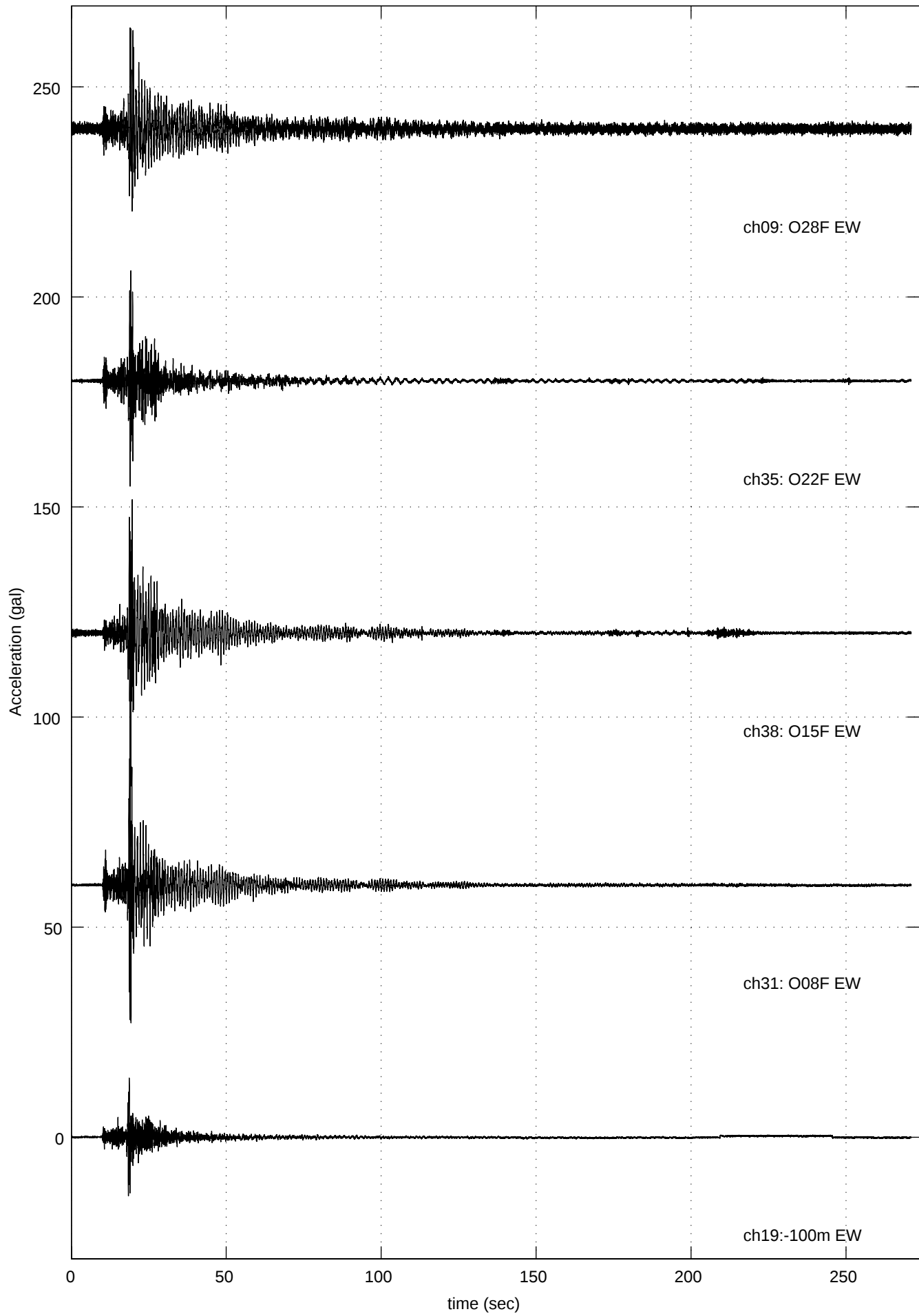
980829 Quake (O28F EW: Max =24 at 18.98 sec )
