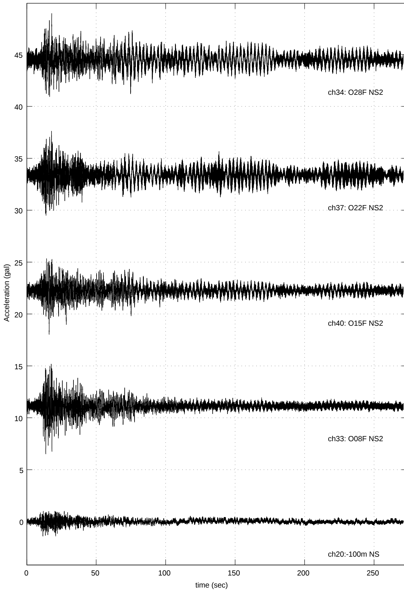
980820 Quake (O28F NS2: Max =4.451 at 17.97 sec )
