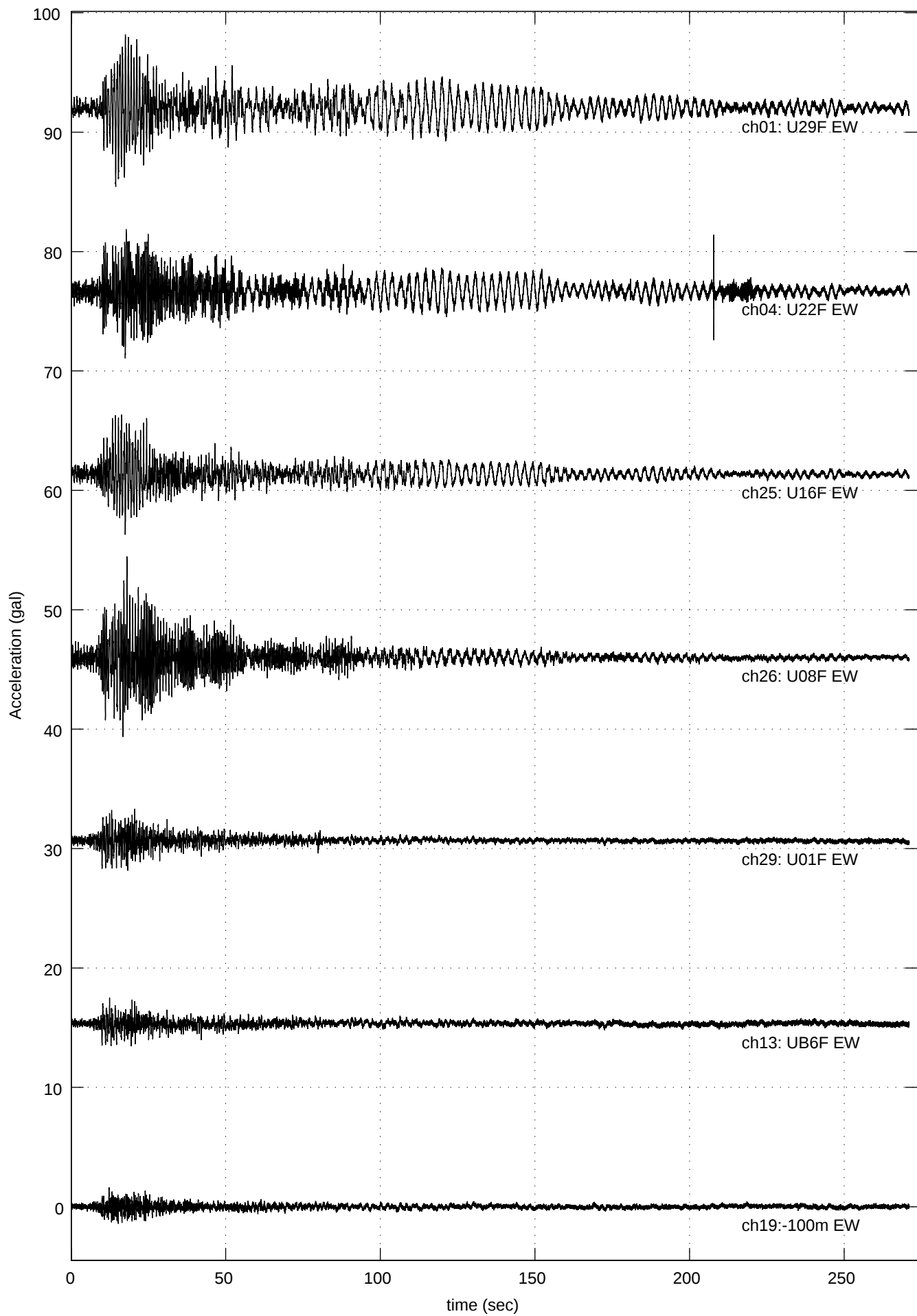
980820 Quake (U29F EW: Max =6.135 at 17.55 sec )
