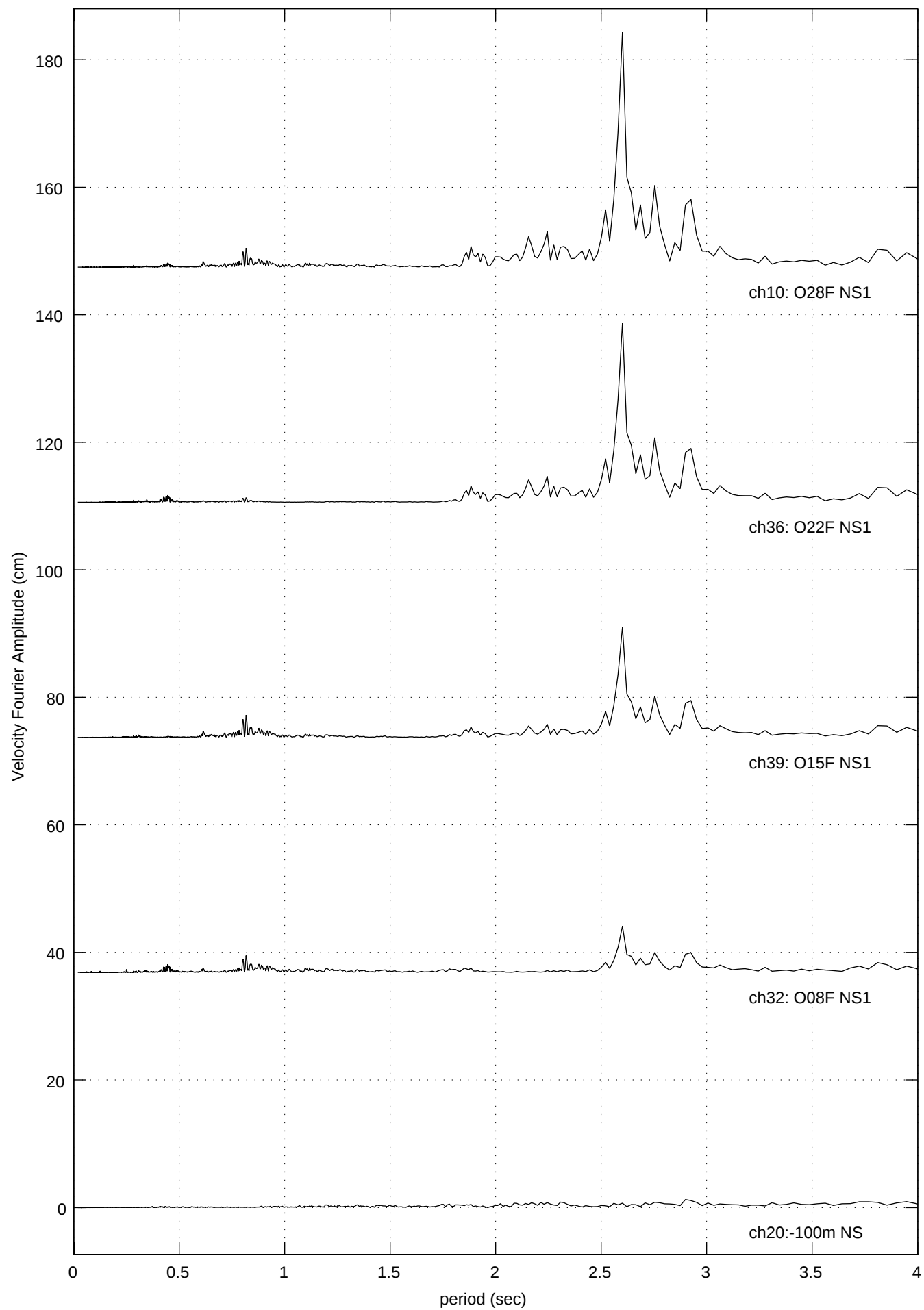
980820 Quake (Office 28F NS1: Max =36.87 at 2.6007 sec )
