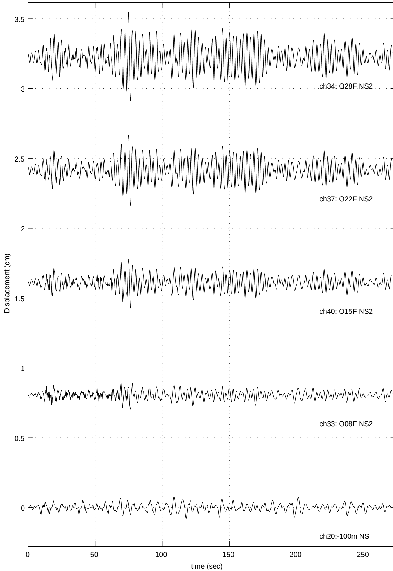
980820 Quake (O28F NS2: Max =0.3222 at 74.81 sec )
