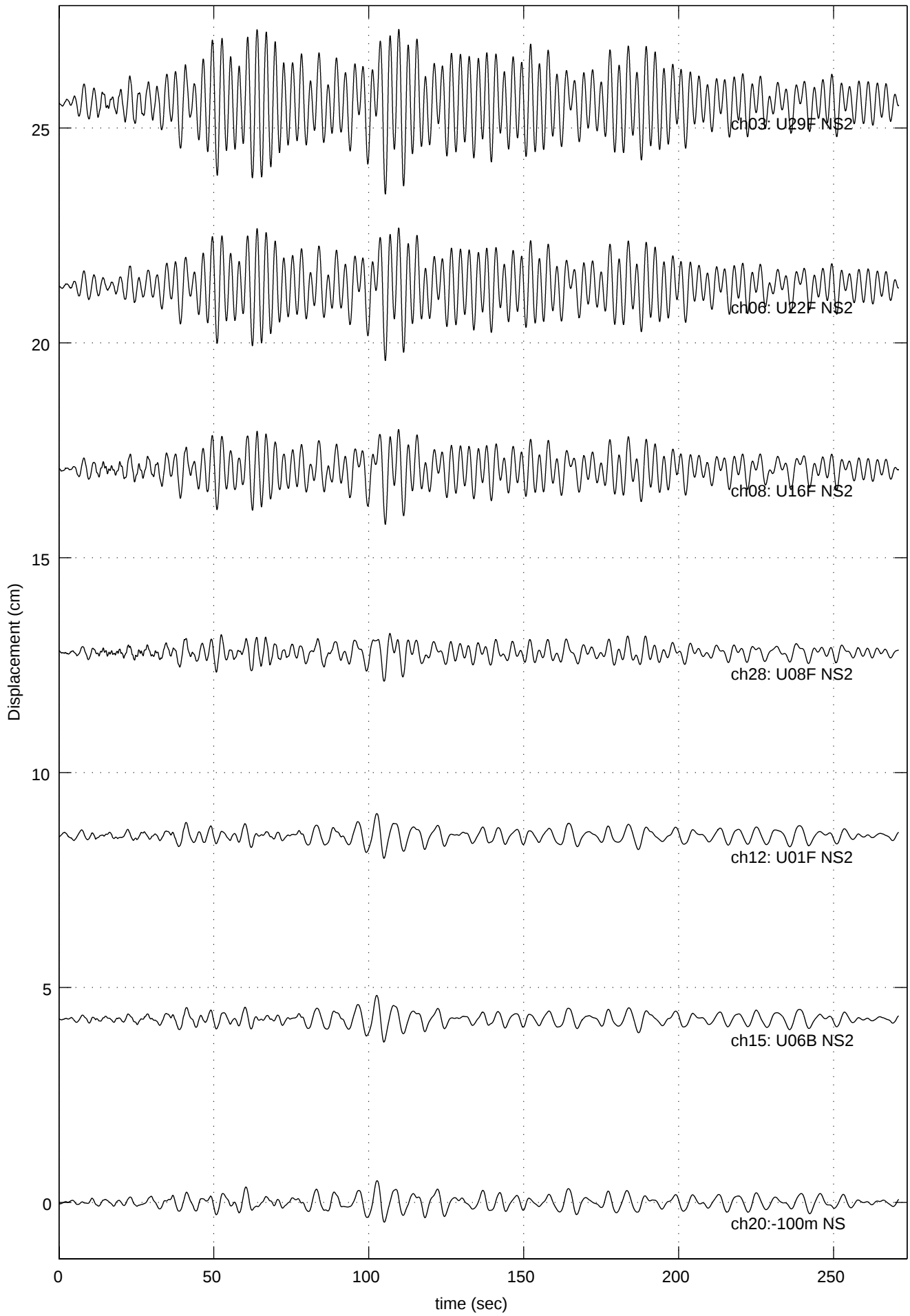
040905-1908 Quake (U29F NS2: Max =1.706 at 109.68 sec )
