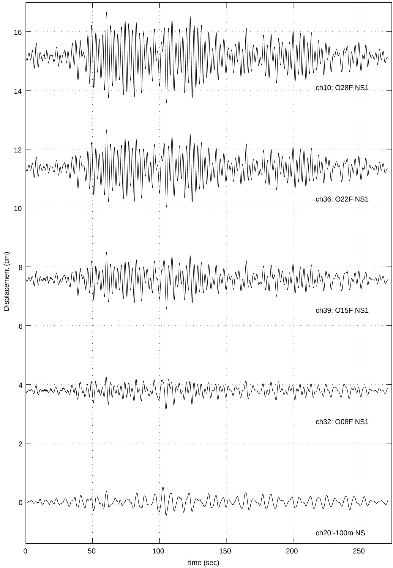
040905-1908 Quake (O28F NS1: Max =1.514 at 60.43 sec )
