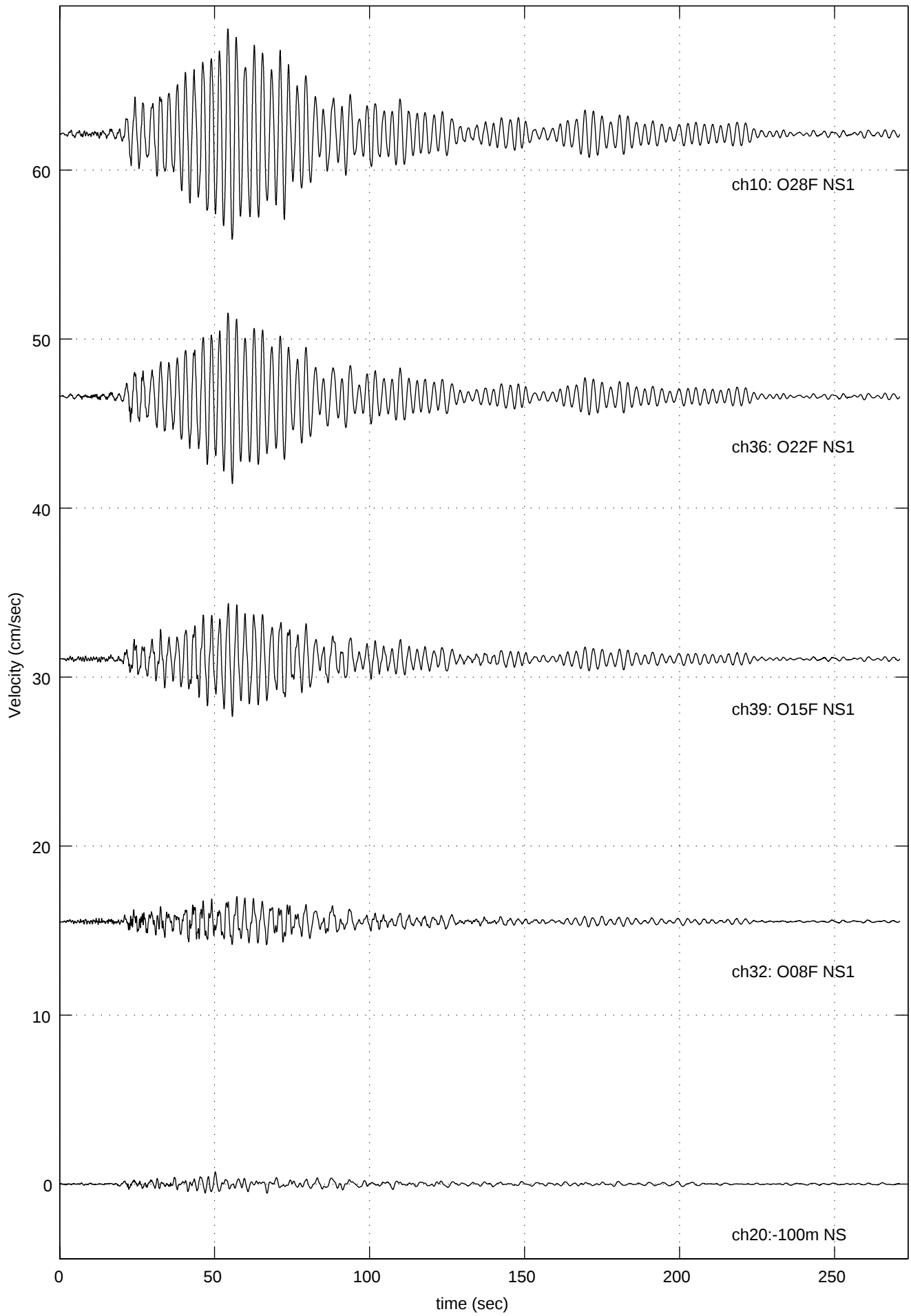
041027-1041 Quake (O28F NS1: Max =6.214 at 54.29 sec )
