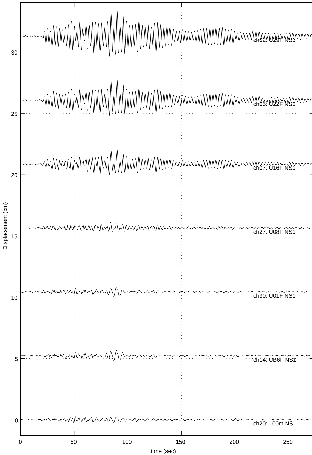
041027-1041 Quake (U29F NS1: Max =2.086 at 89.85 sec )
