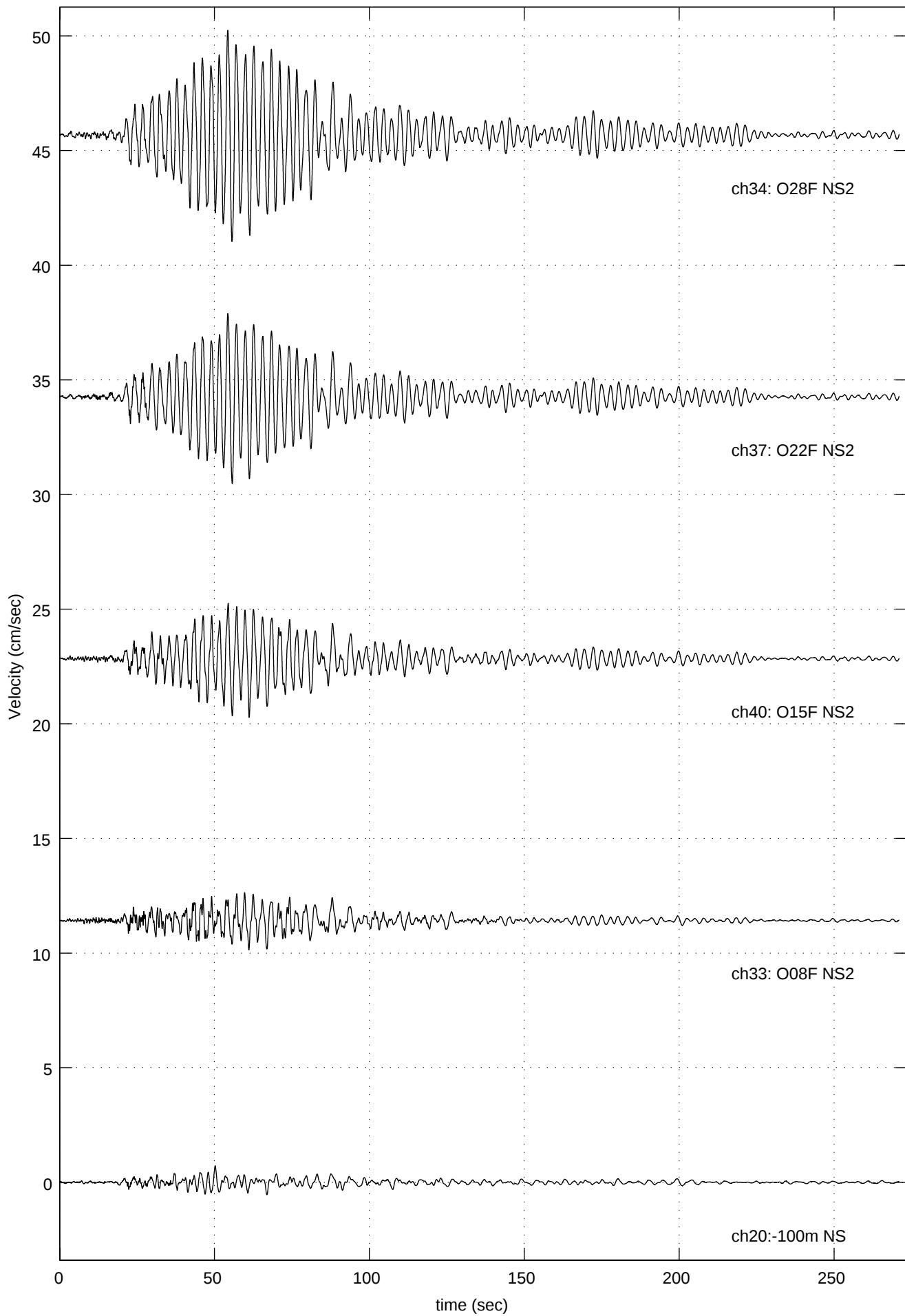
041027-1041 Quake (O28F NS2: Max =4.568 at 54.28 sec )
