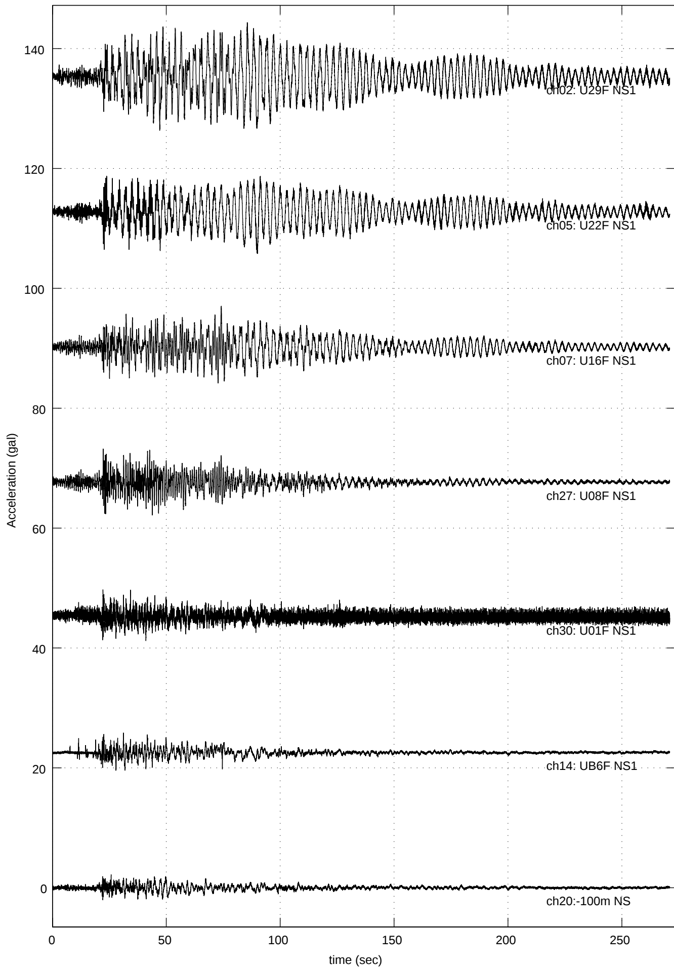
041027-1041 Quake (U29F NS1: Max =9.021 at 85.52 sec )
