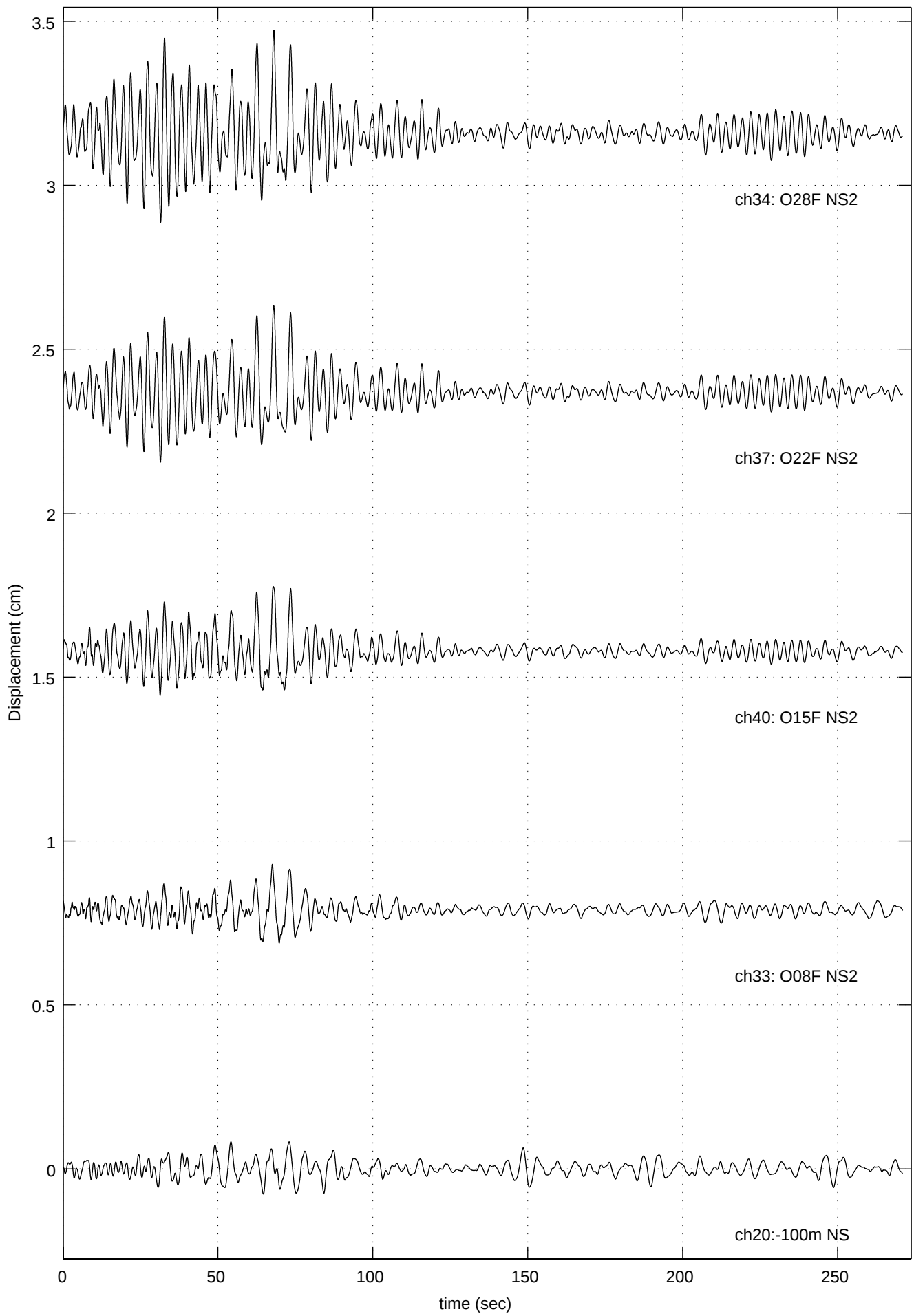
041023-1947 Quake (O28F NS2: Max =0.3158 at 68.03 sec )
