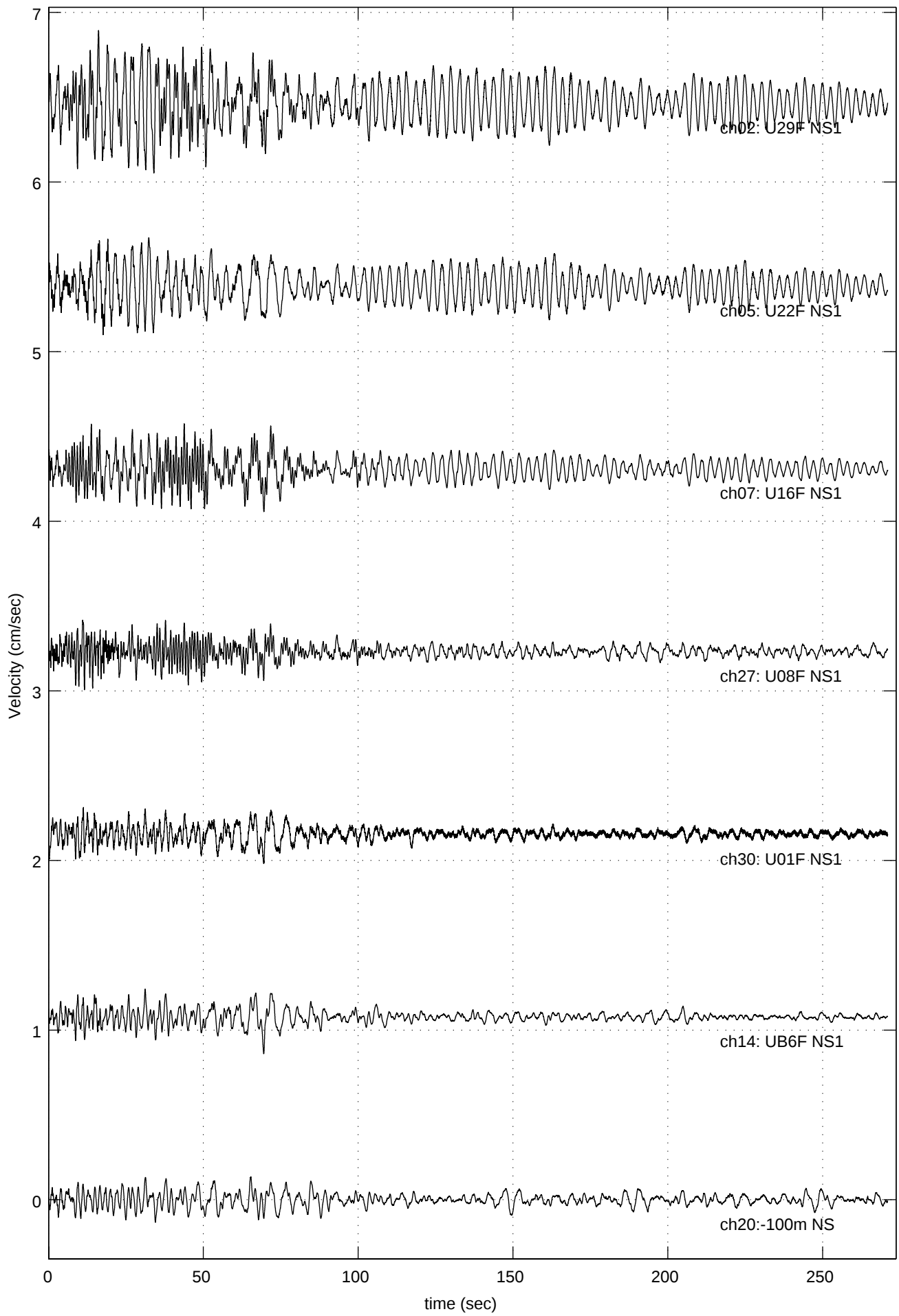
041023-1947 Quake (U29F NS1: Max =0.4308 at 16.18 sec )
