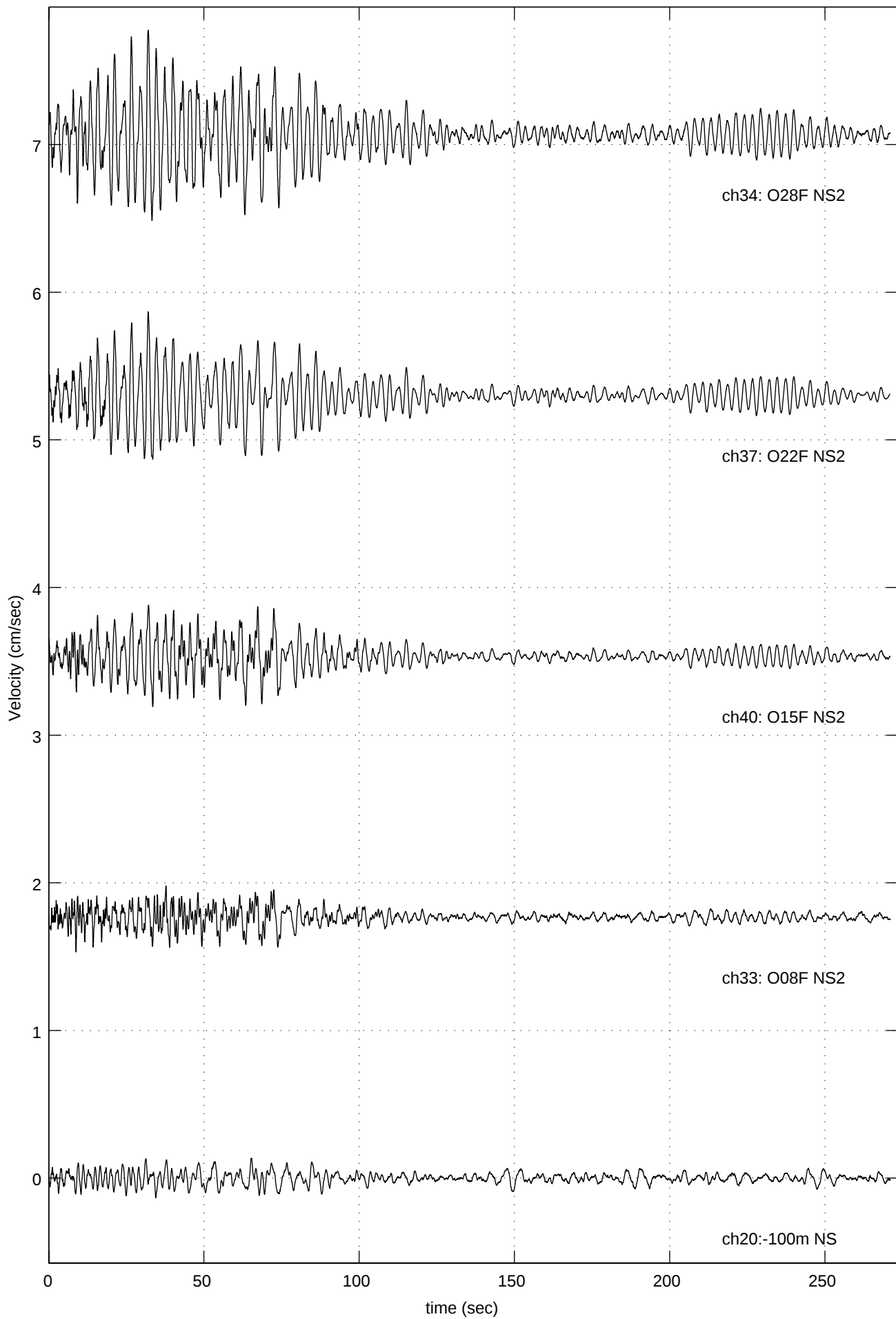
041023-1947 Quake (O28F NS2: Max =0.7068 at 32.07 sec )
