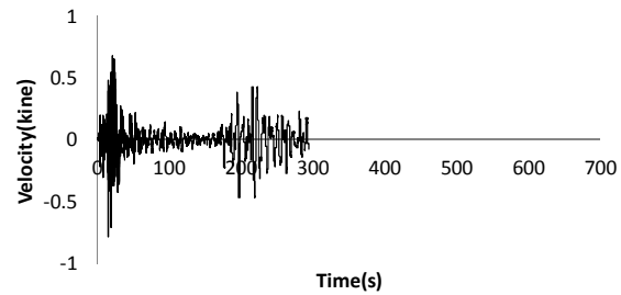
80302E02-1FLN330E-VEL
