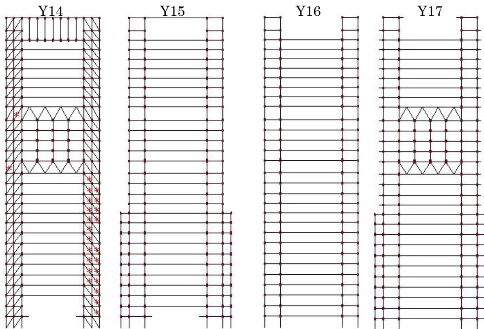
Ai-EW 層間変形角 1/75
