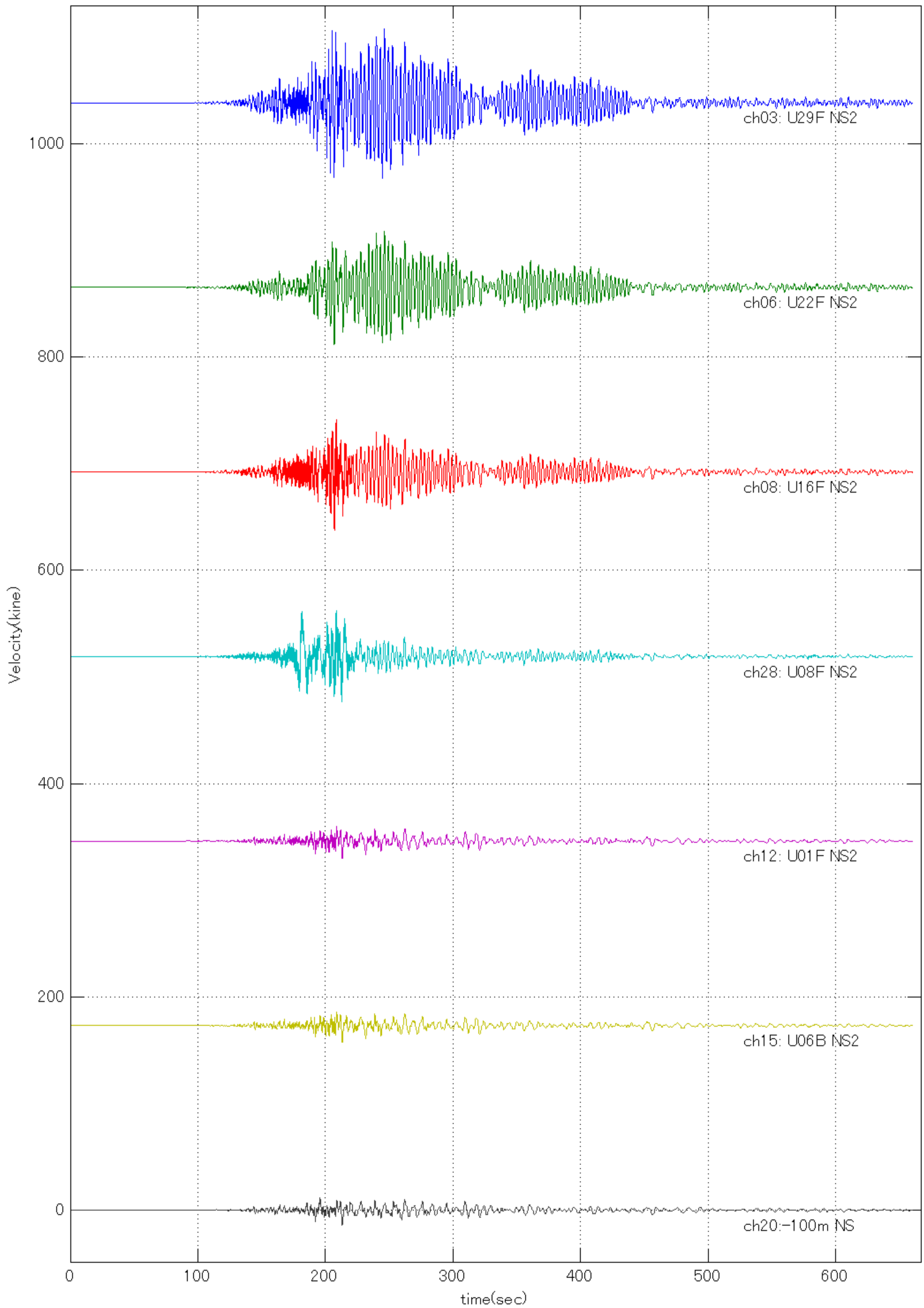
20110311144600 Quake (U29F NS2: Max =69.2188 at 246.18 sec )
