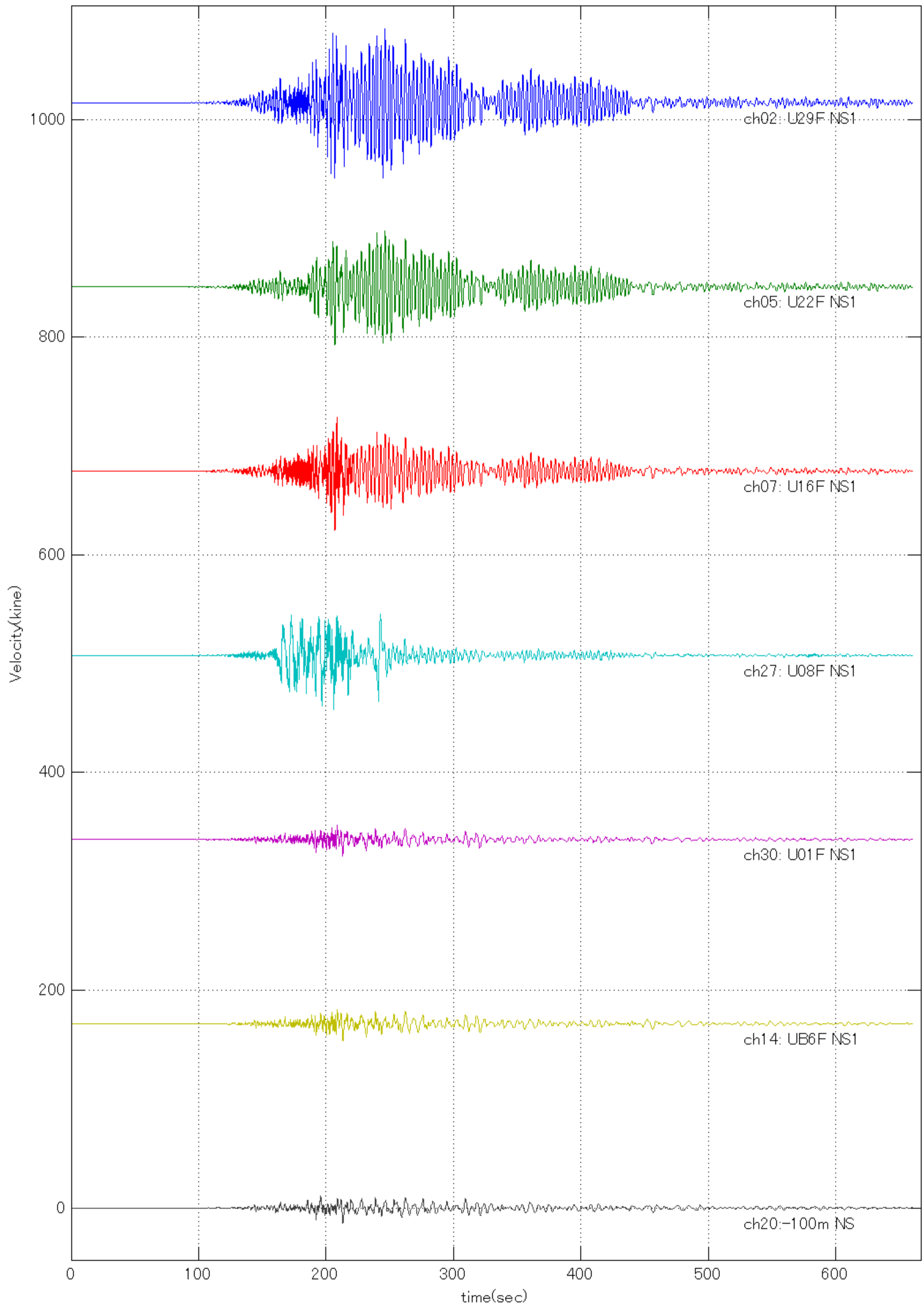
20110311144600 Quake (U29F NS1: Max =67.6853 at 246.15 sec )
