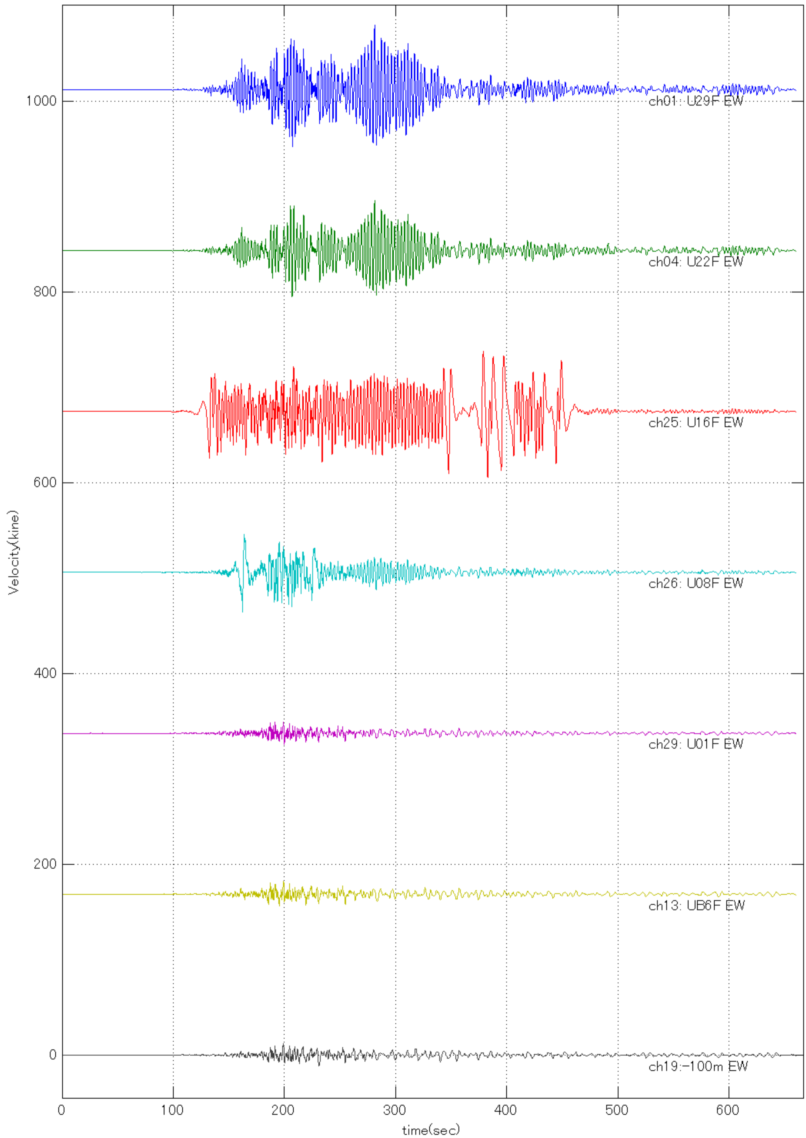
20110311144600 Quake (U29F EW: Max =67.4749 at 281.18 sec )
