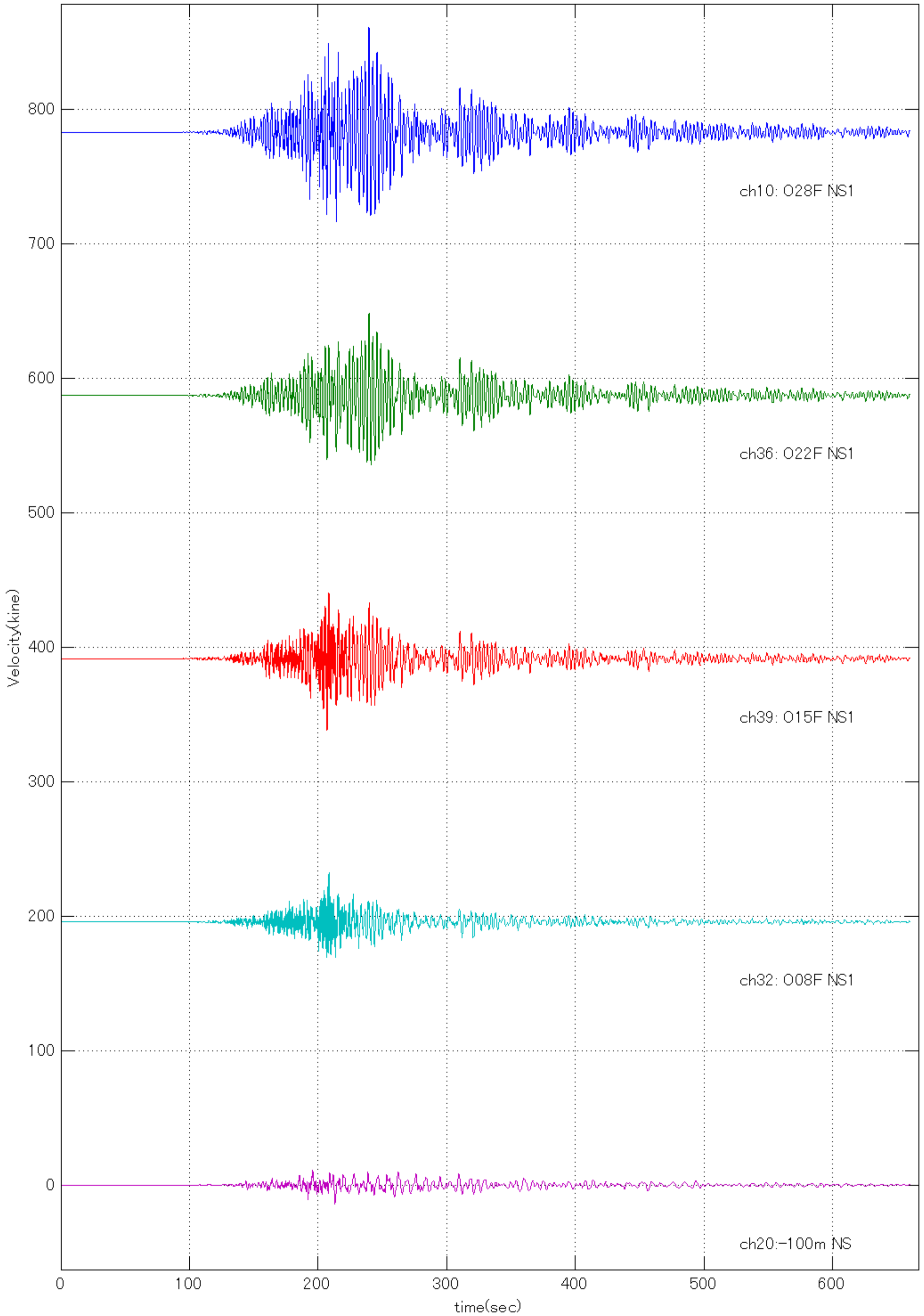
20110311144600 Quake (O28F NS1: Max =78.2907 at 239.46 sec )
