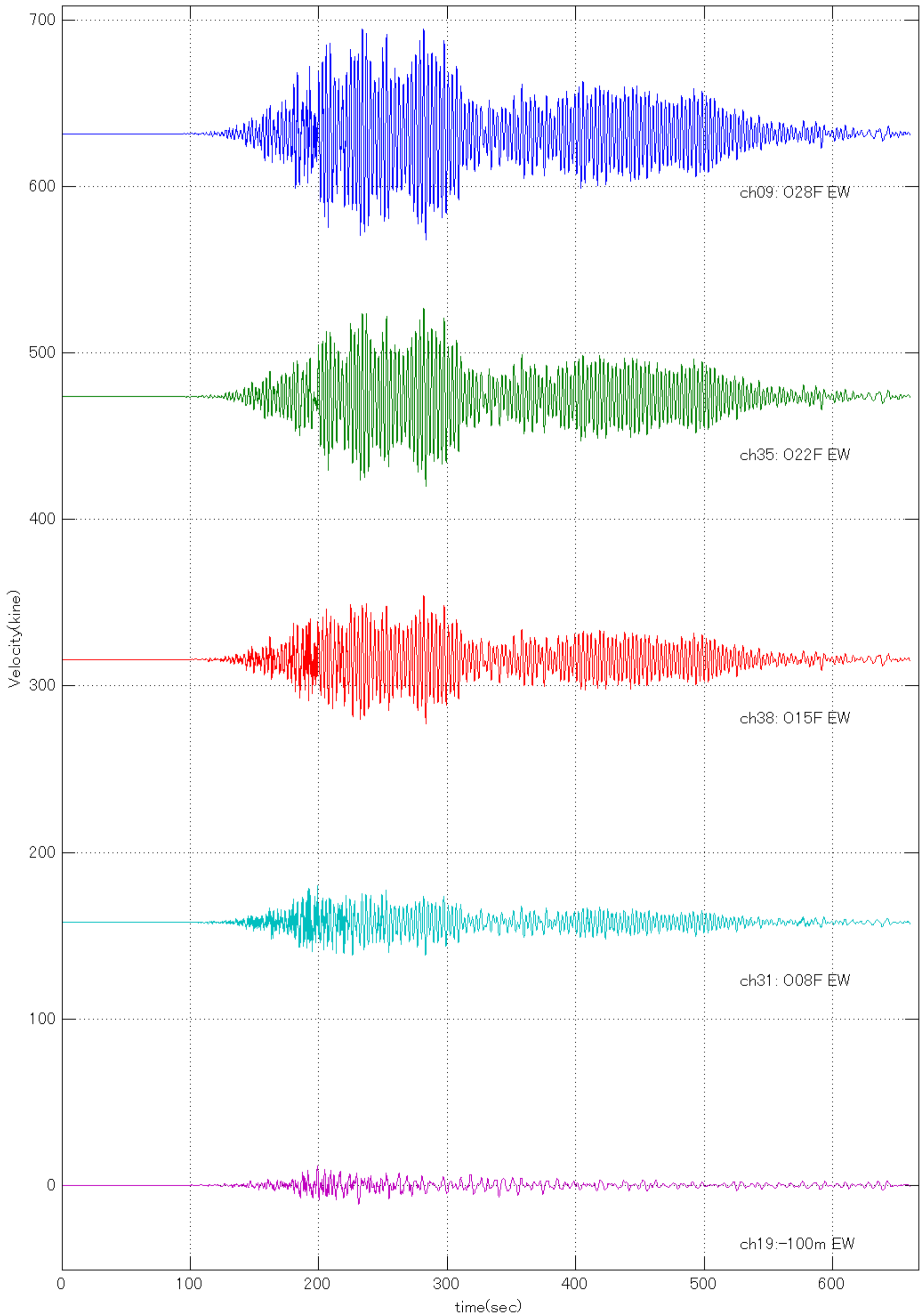
20110311144600 Quake (O28F EW: Max =63.1659 at 233.91 sec )
