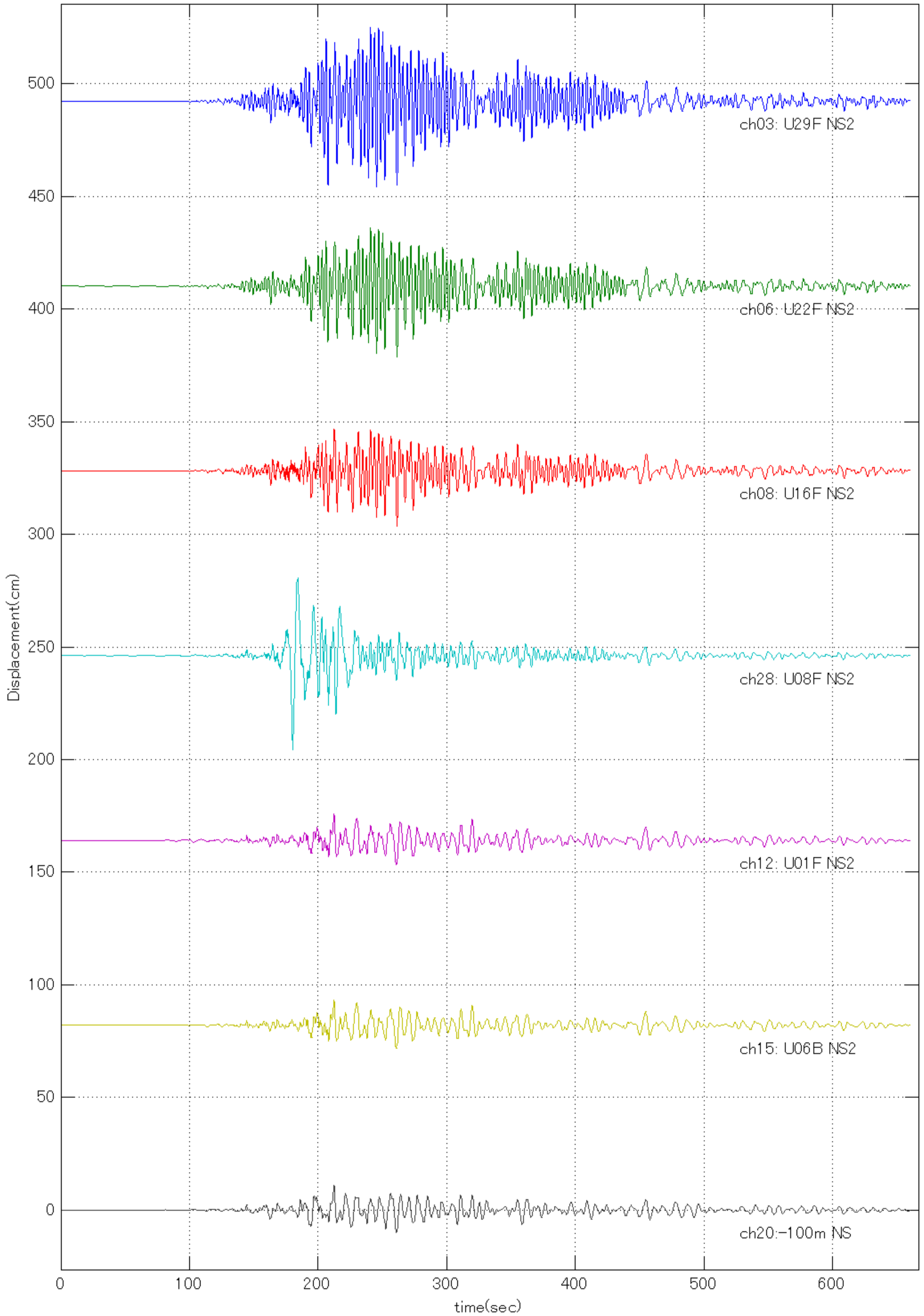
20110311144600 Quake (U29F NS2: Max =32.8131 at 240.65 sec )
