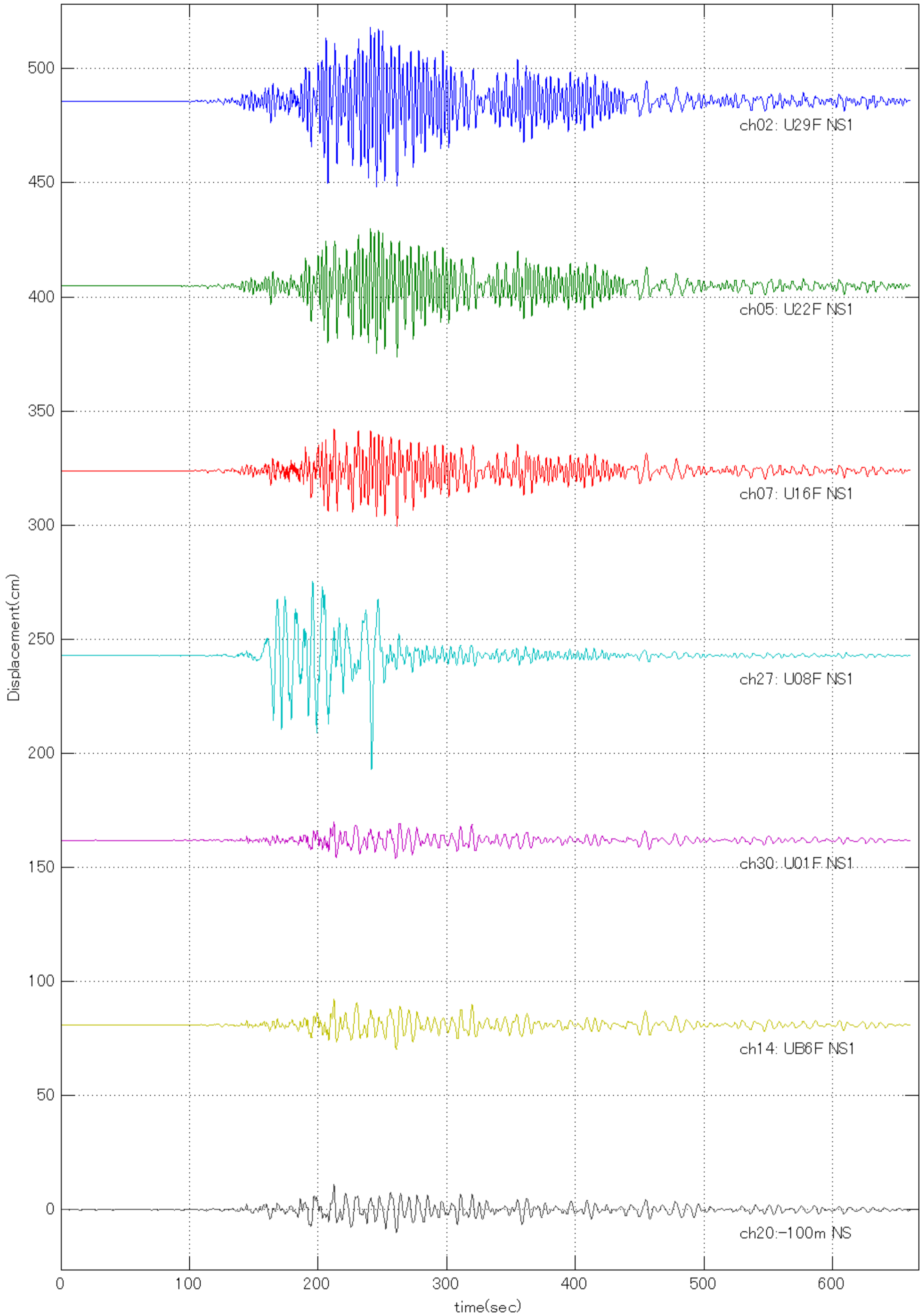
20110311144600 Quake (U29F NS1: Max =32.3782 at 240.65 sec )
