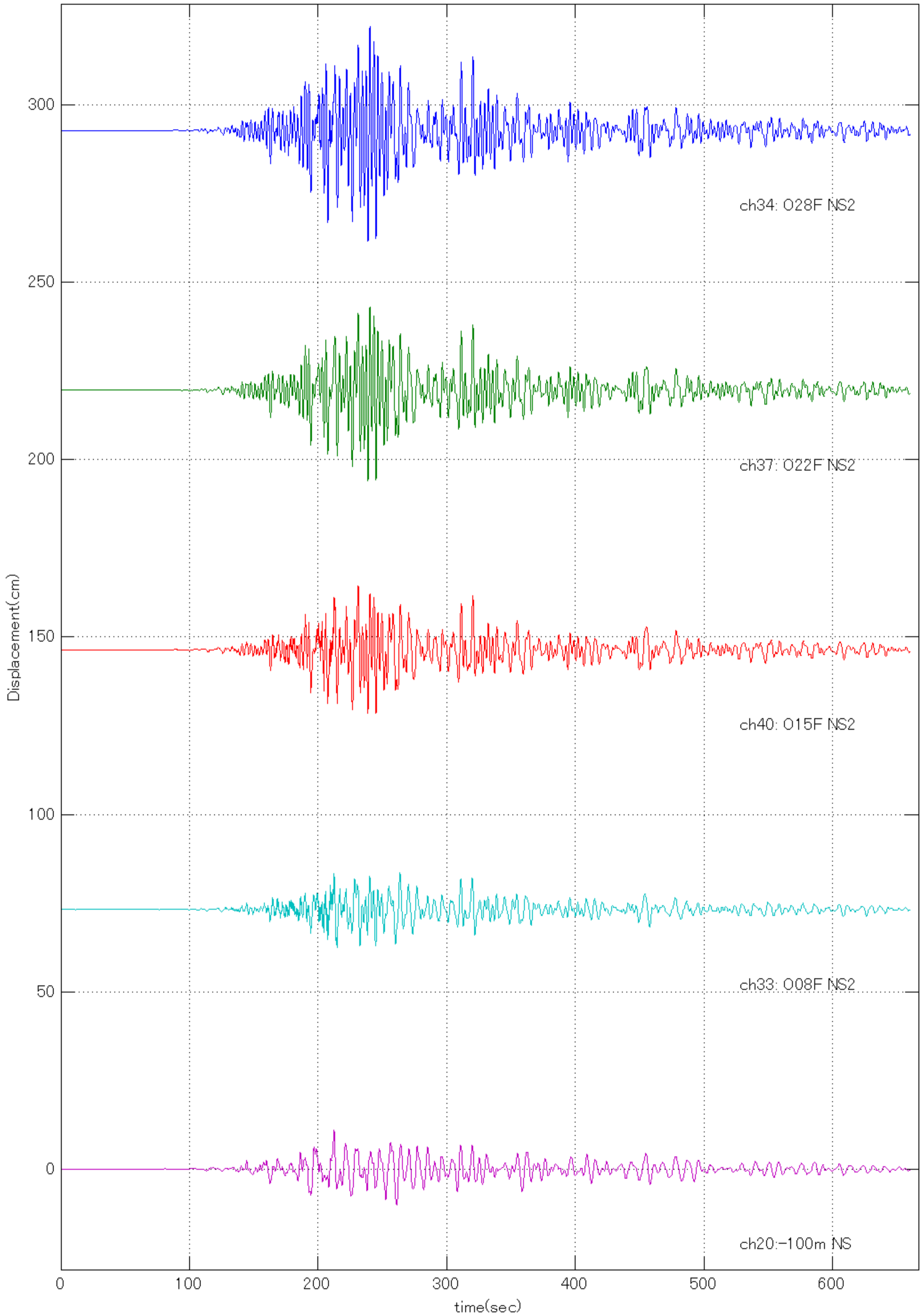
20110311144600 Quake (O28F NS2: Max =29.2784 at 240.29 sec )
