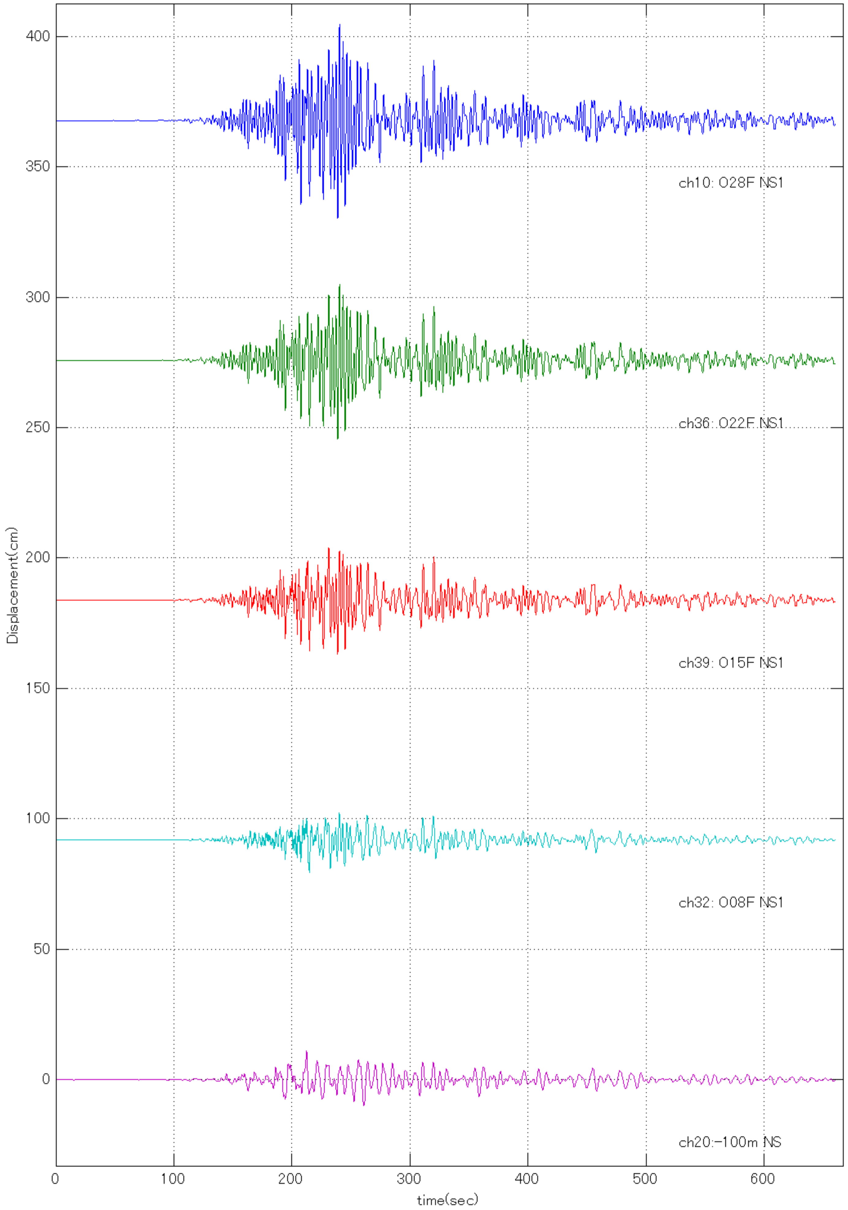
20110311144600 Quake (O28F NS1: Max =36.7726 at 240.31 sec )
