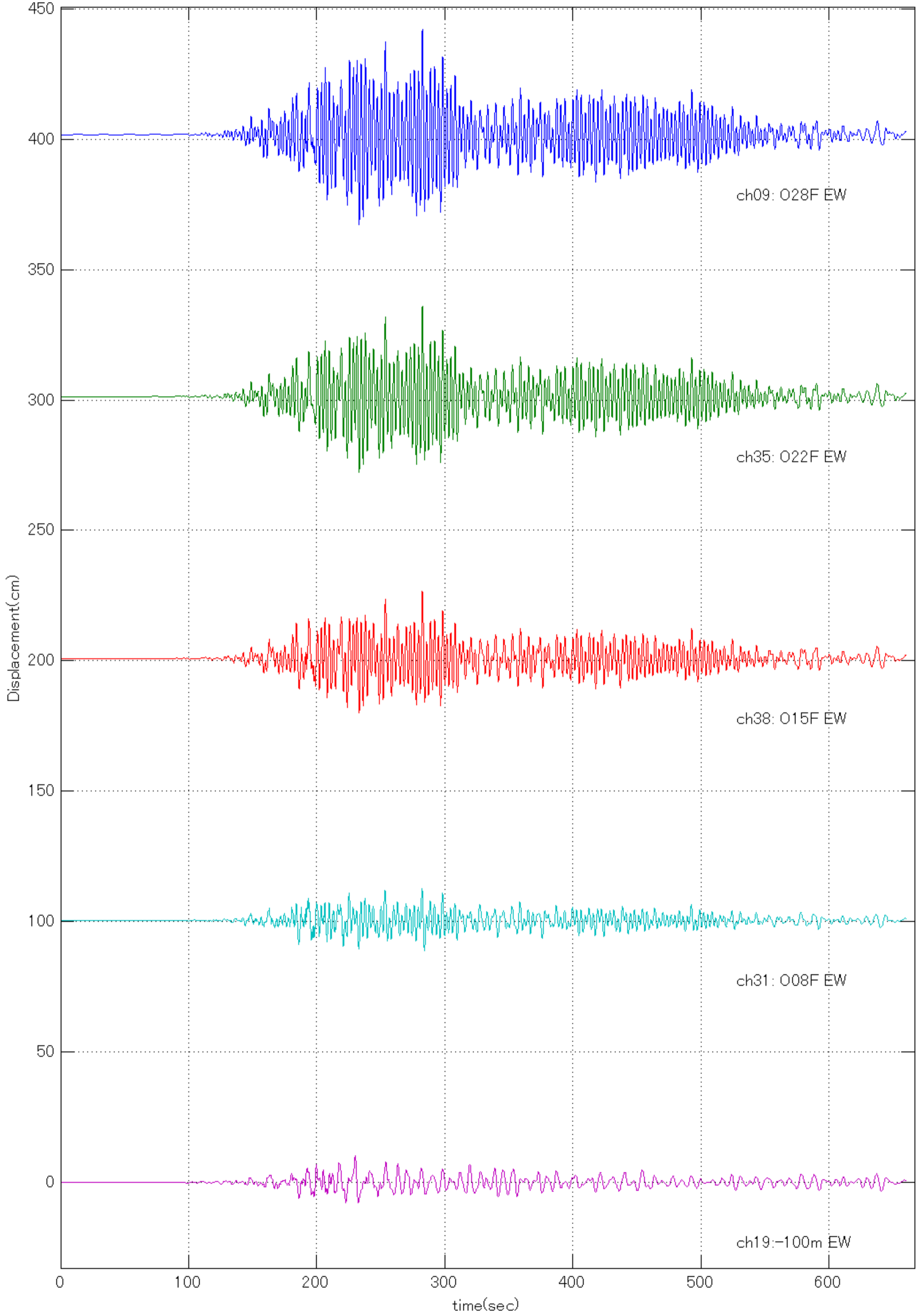
20110311144600 Quake (O28F EW: Max =40.1767 at 282.5 sec )
