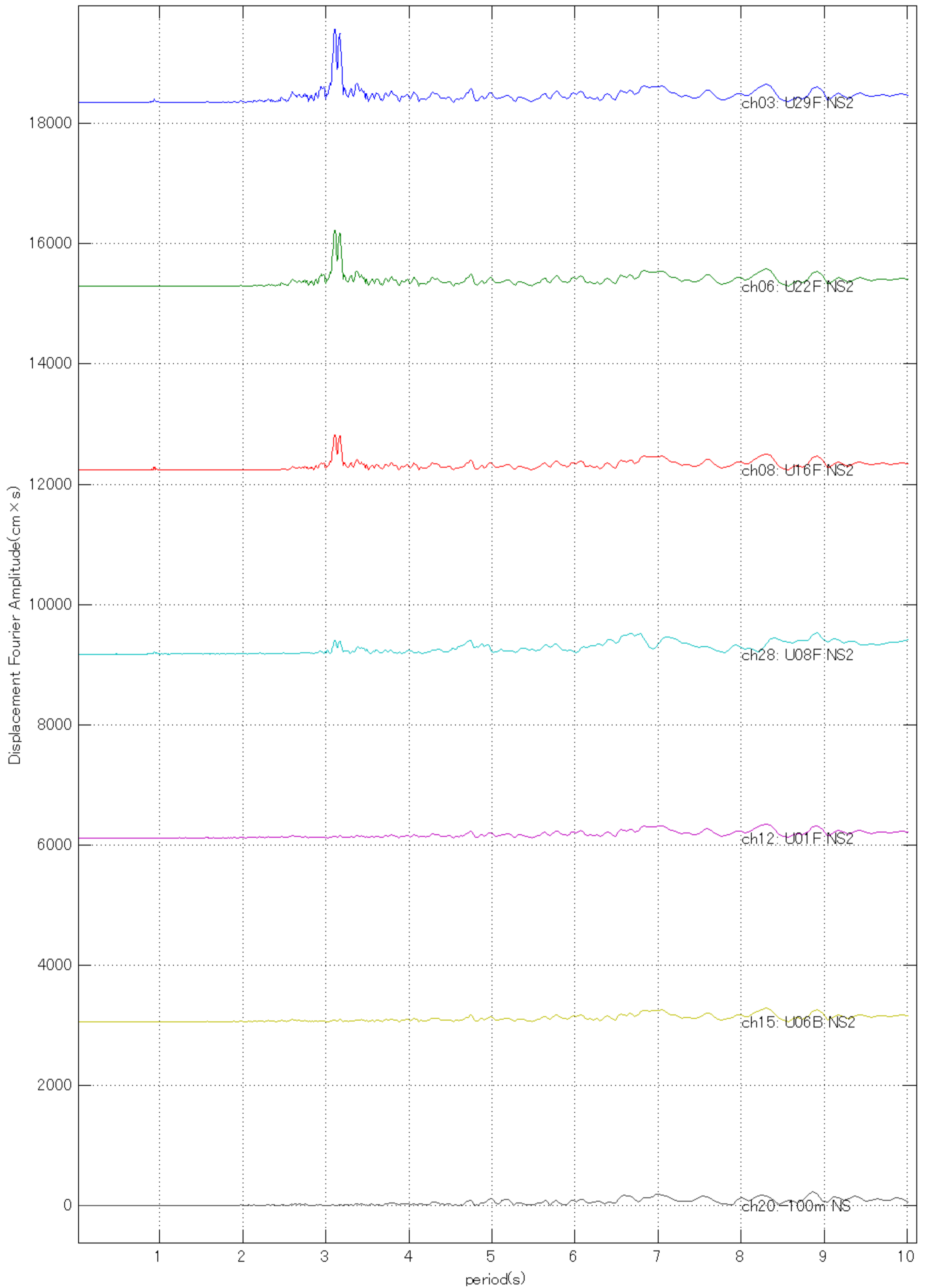
20110311144600 Quake (U29F NS2: Max =1223.4169 at 3.106 sec )
