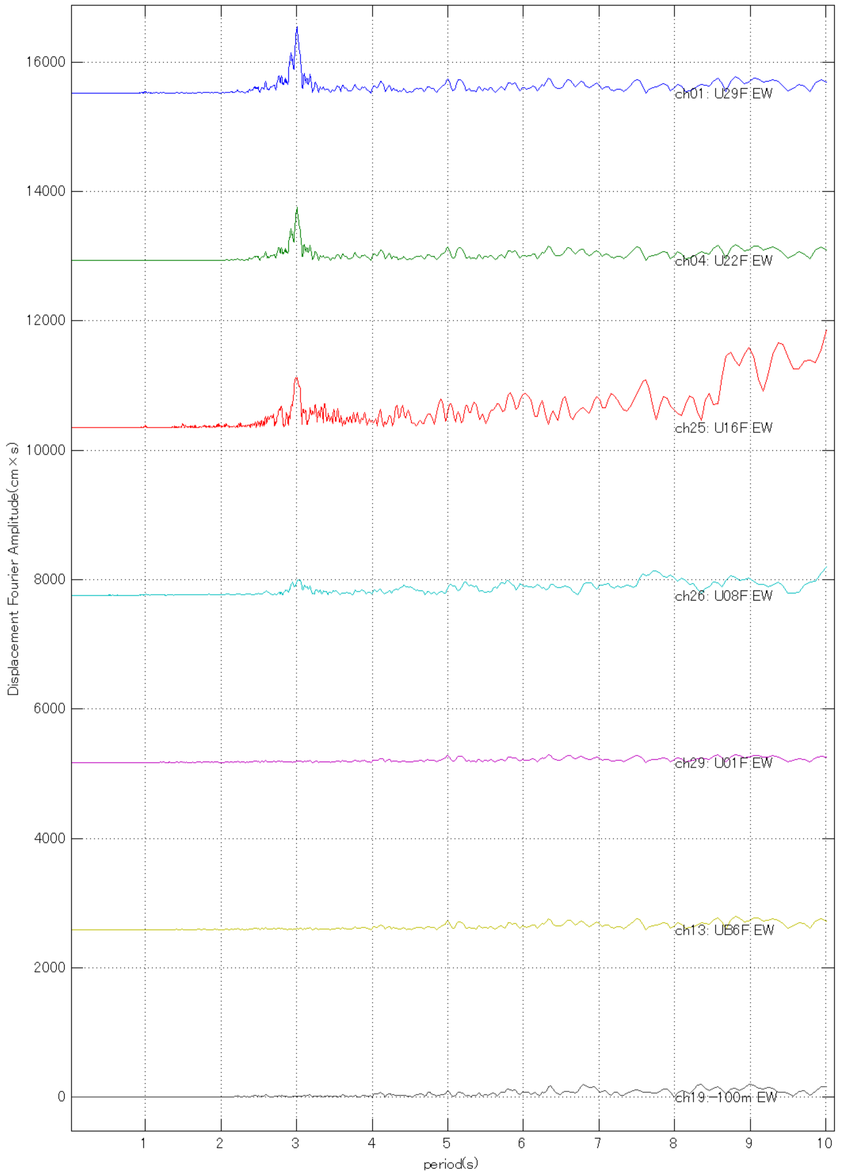
20110311144600 Quake (U29F EW: Max =1034.6894 at 3.0062 sec )
