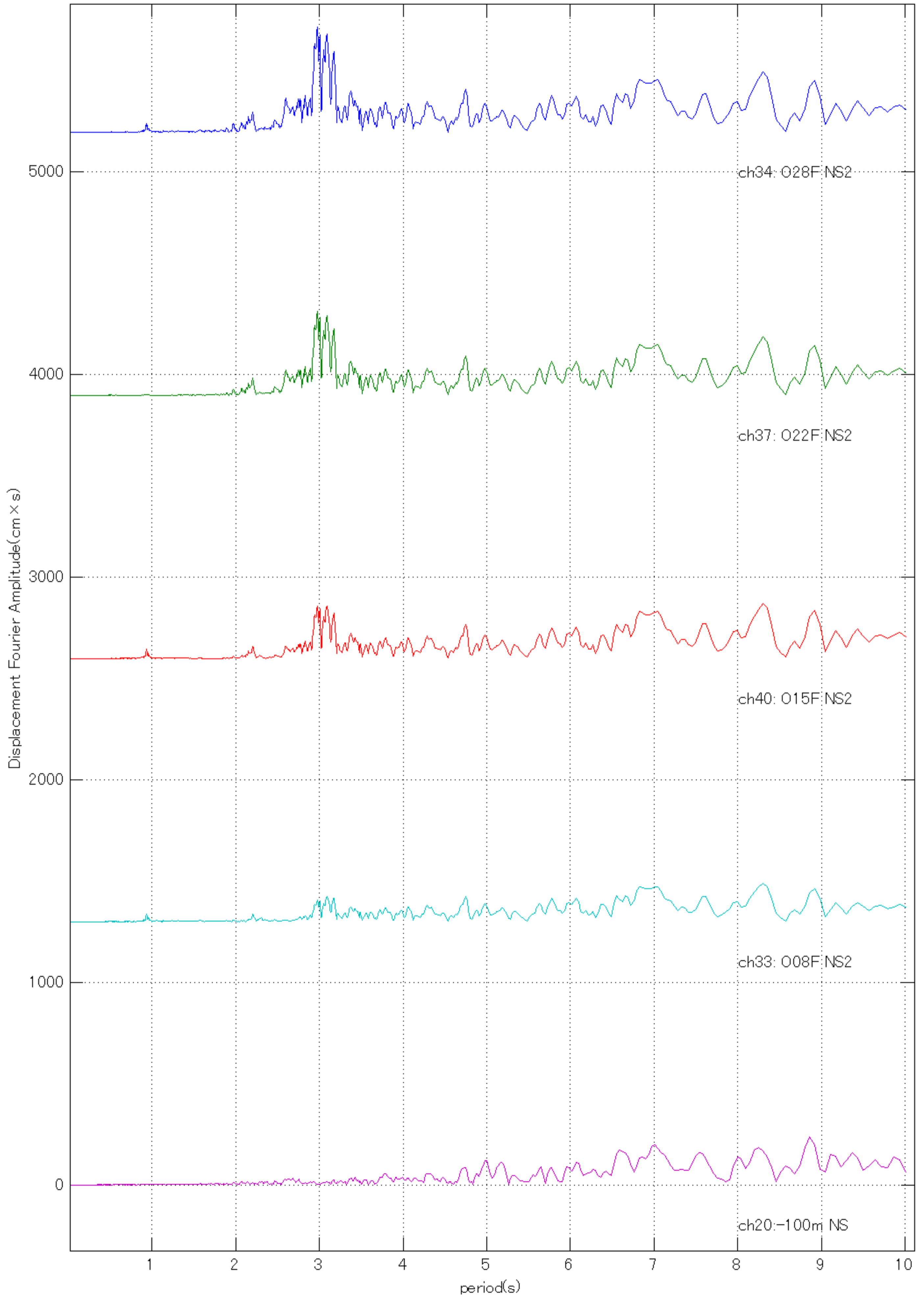
20110311144600 Quake (O28F NS2: Max =519.7293 at 2.9789 sec )
