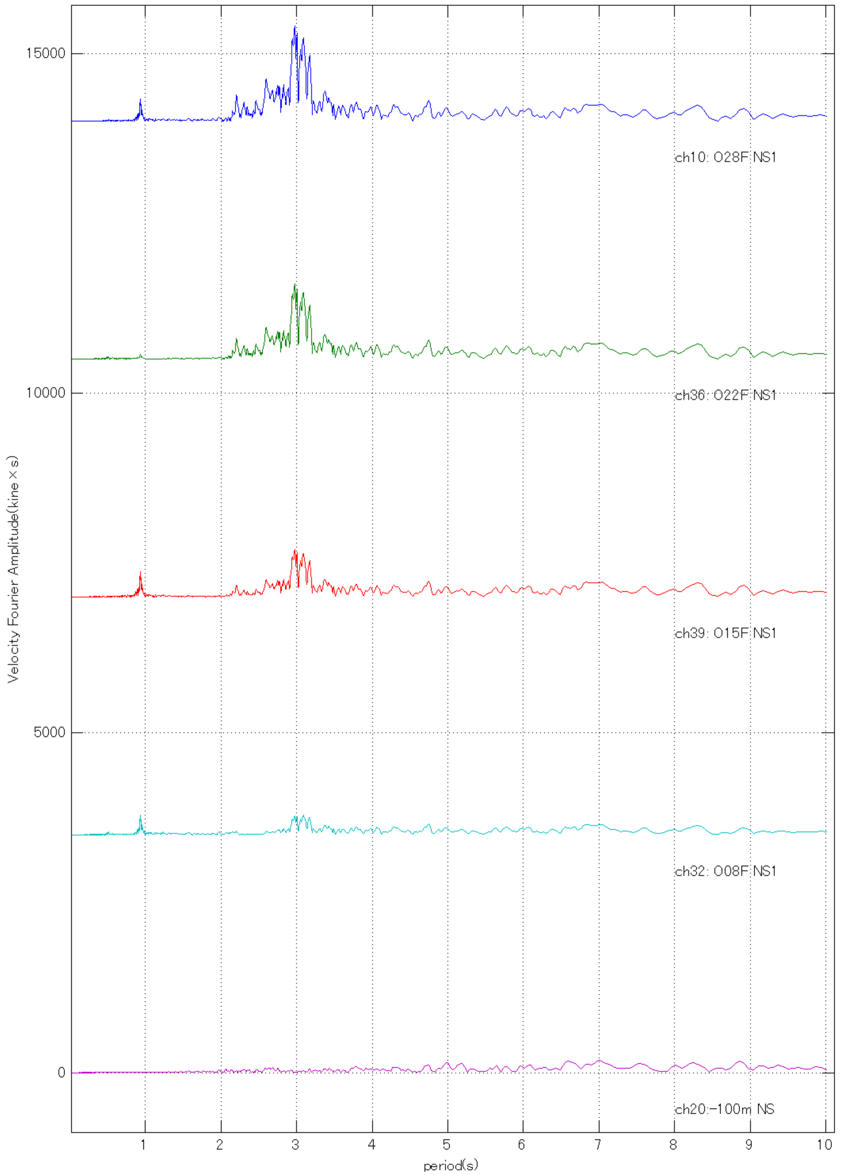
20110311144600 Quake (O28F NS1: Max =1401.2846 at 2.9789 sec )
