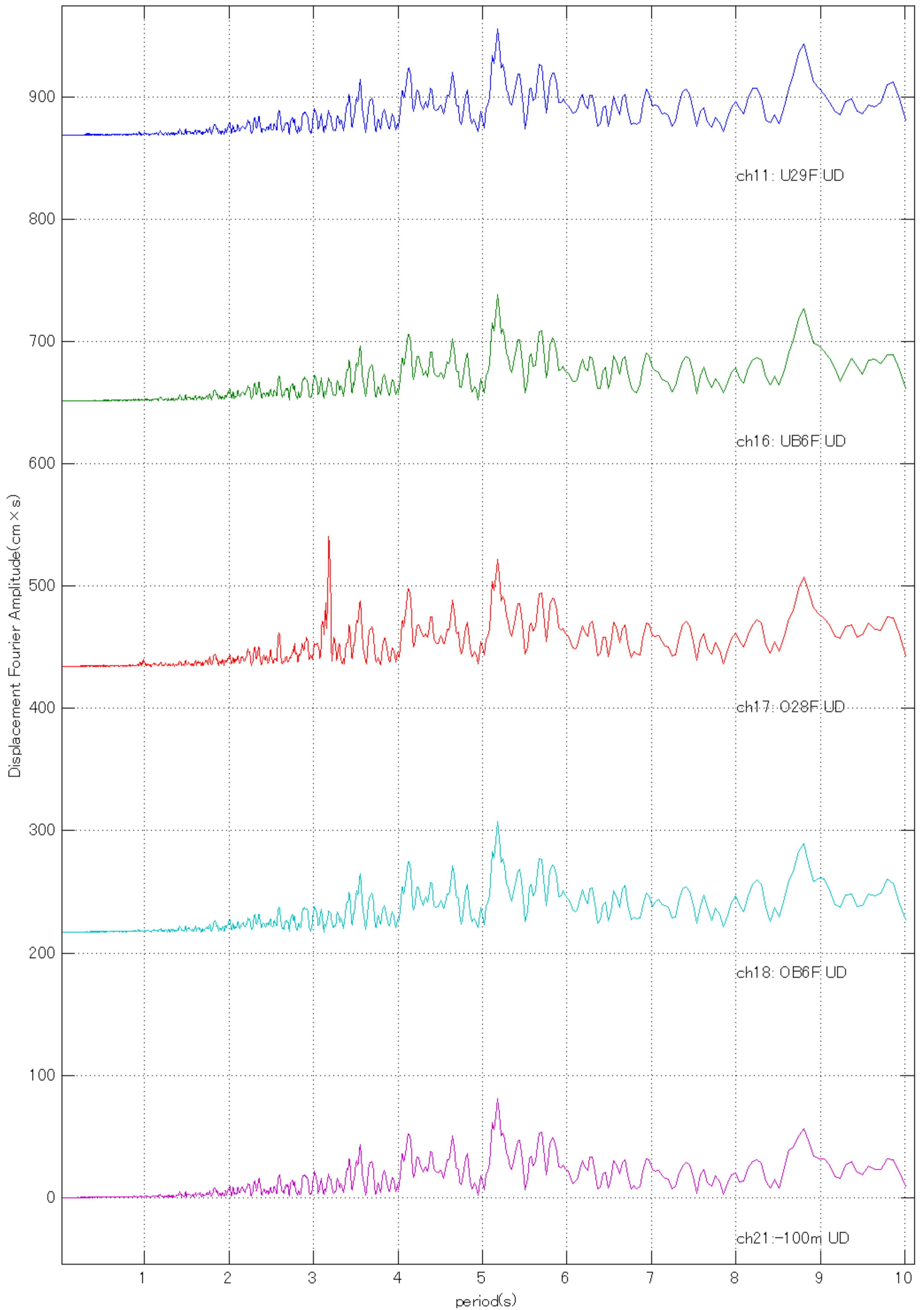
20110311144600 Quake (University 29F UD: Max =86.9267 at 5.1807 sec )
