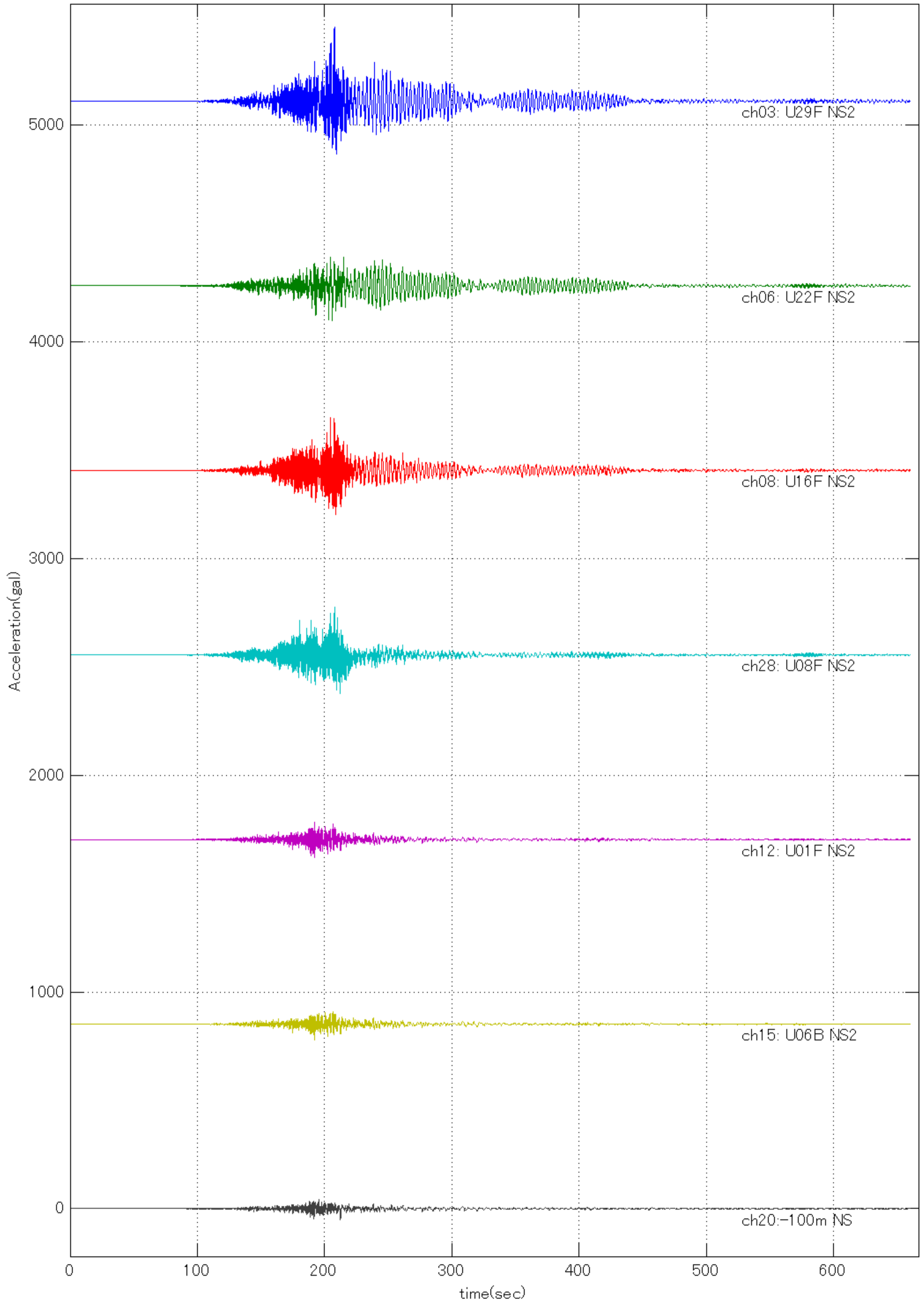
20110311144600 Quake (U29F NS2: Max =340.7469 at 207.69 sec )
