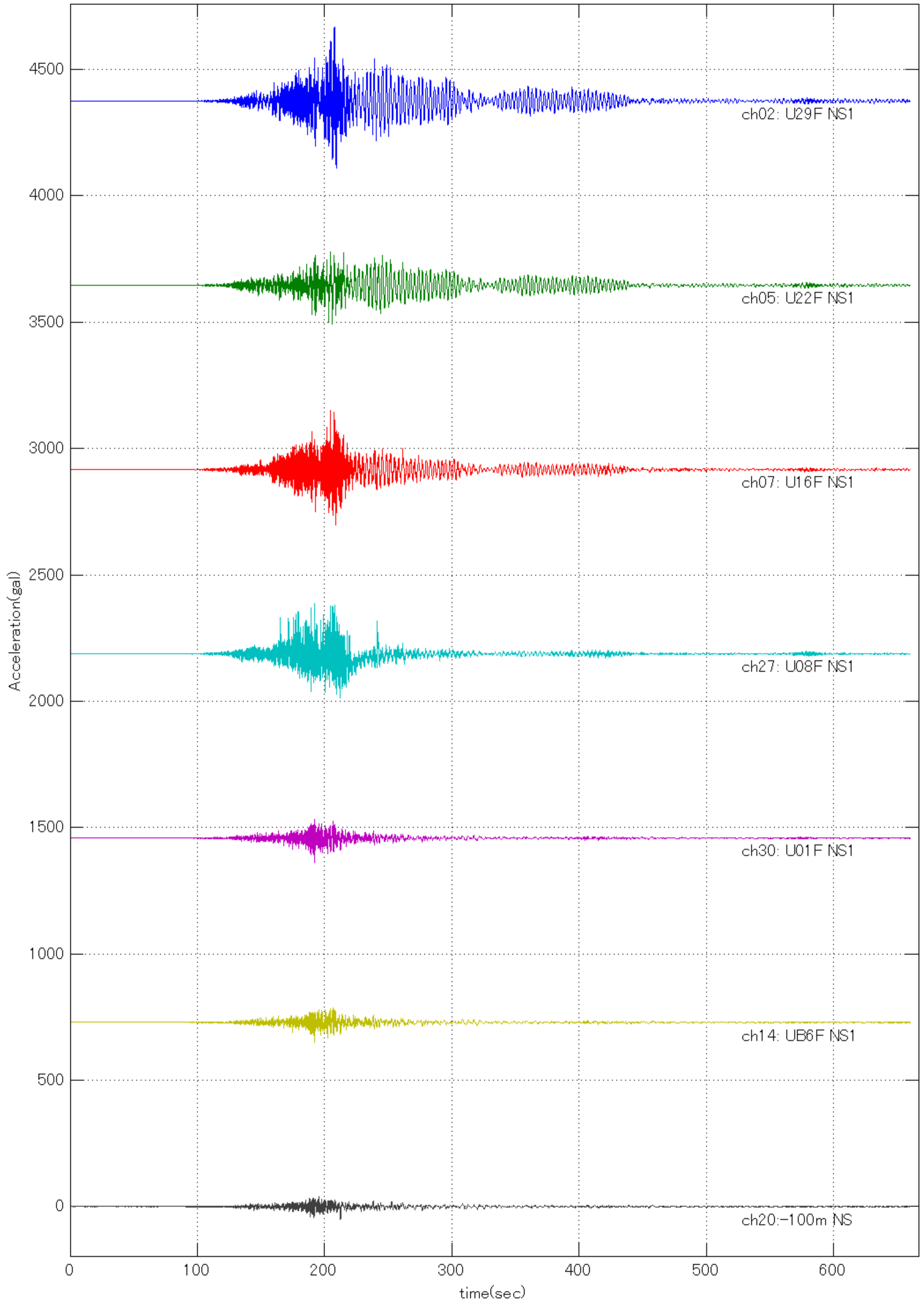
20110311144600 Quake (U29F NS1: Max =291.6487 at 207.69 sec )
