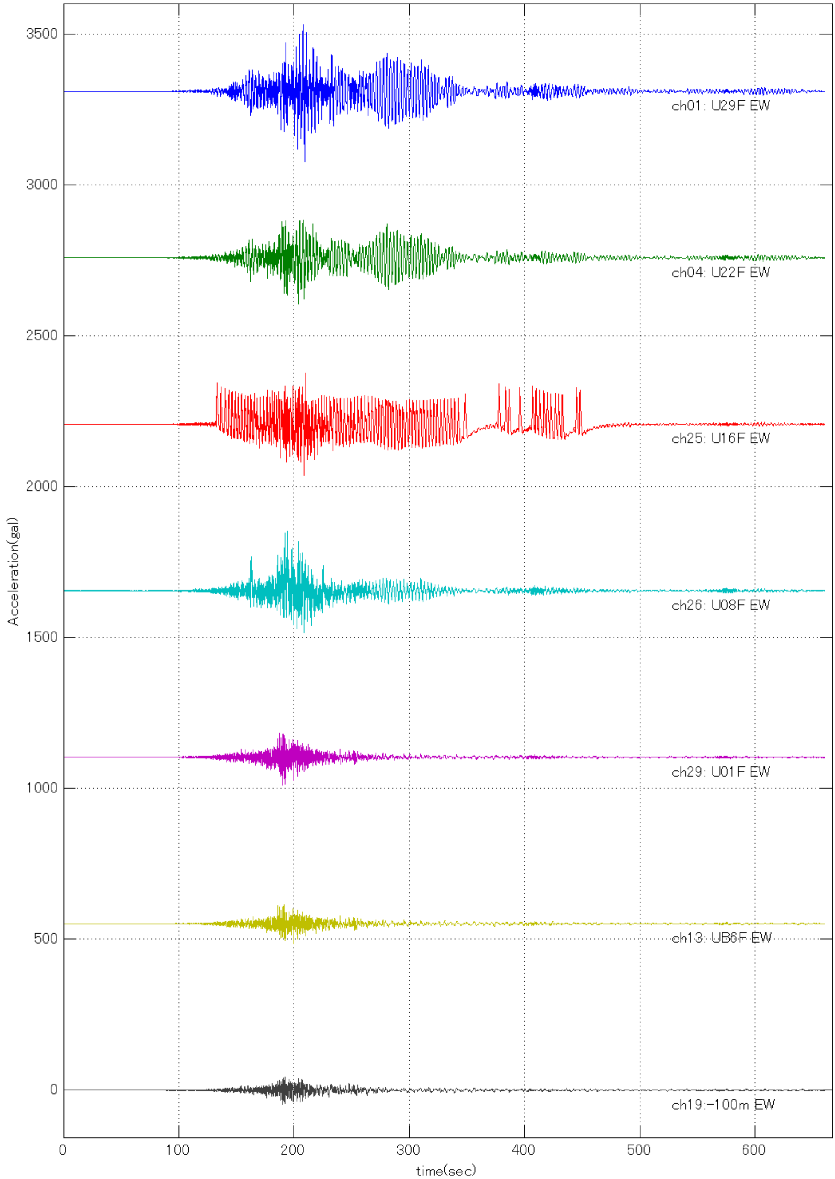
20110311144600 Quake (U29F EW: Max =220.6835 at 207.73 sec )
