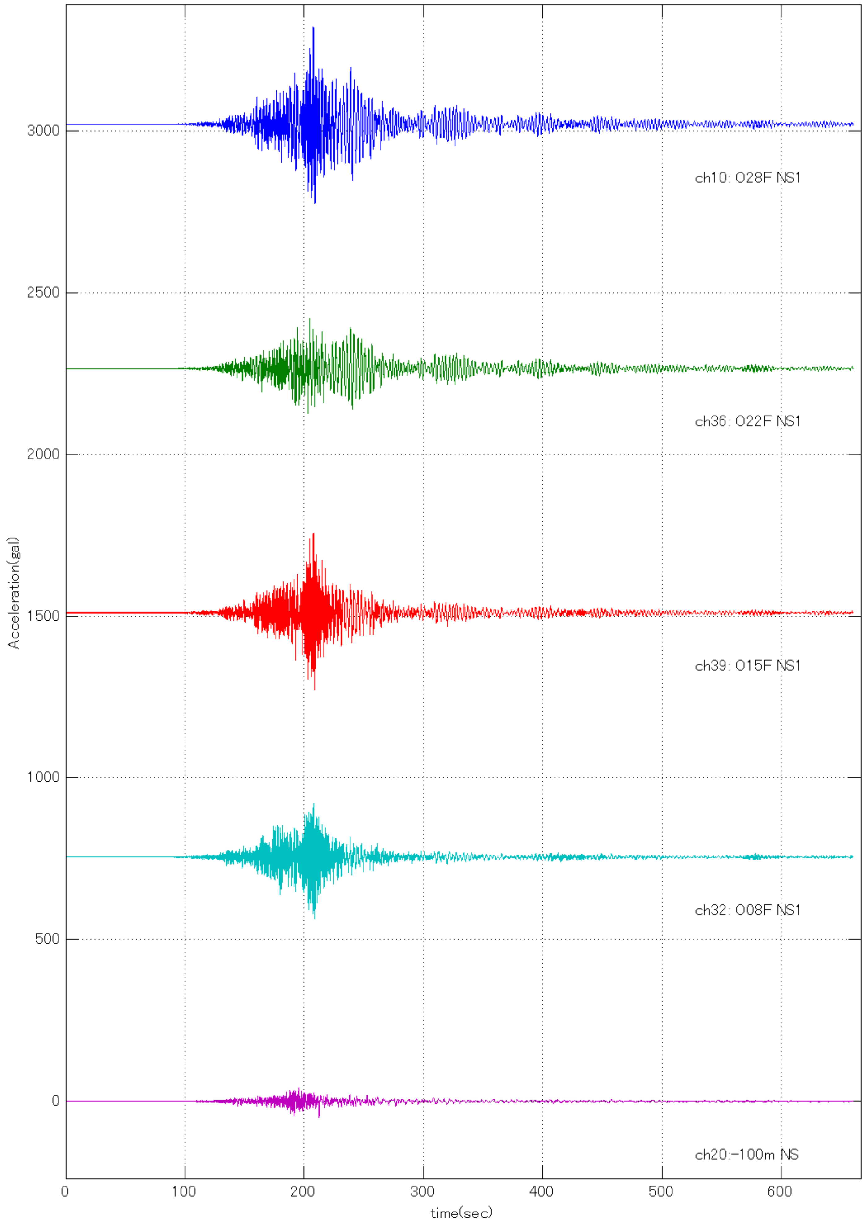
20110311144600 Quake (O28F NS1: Max =302.0577 at 207.67 sec )
