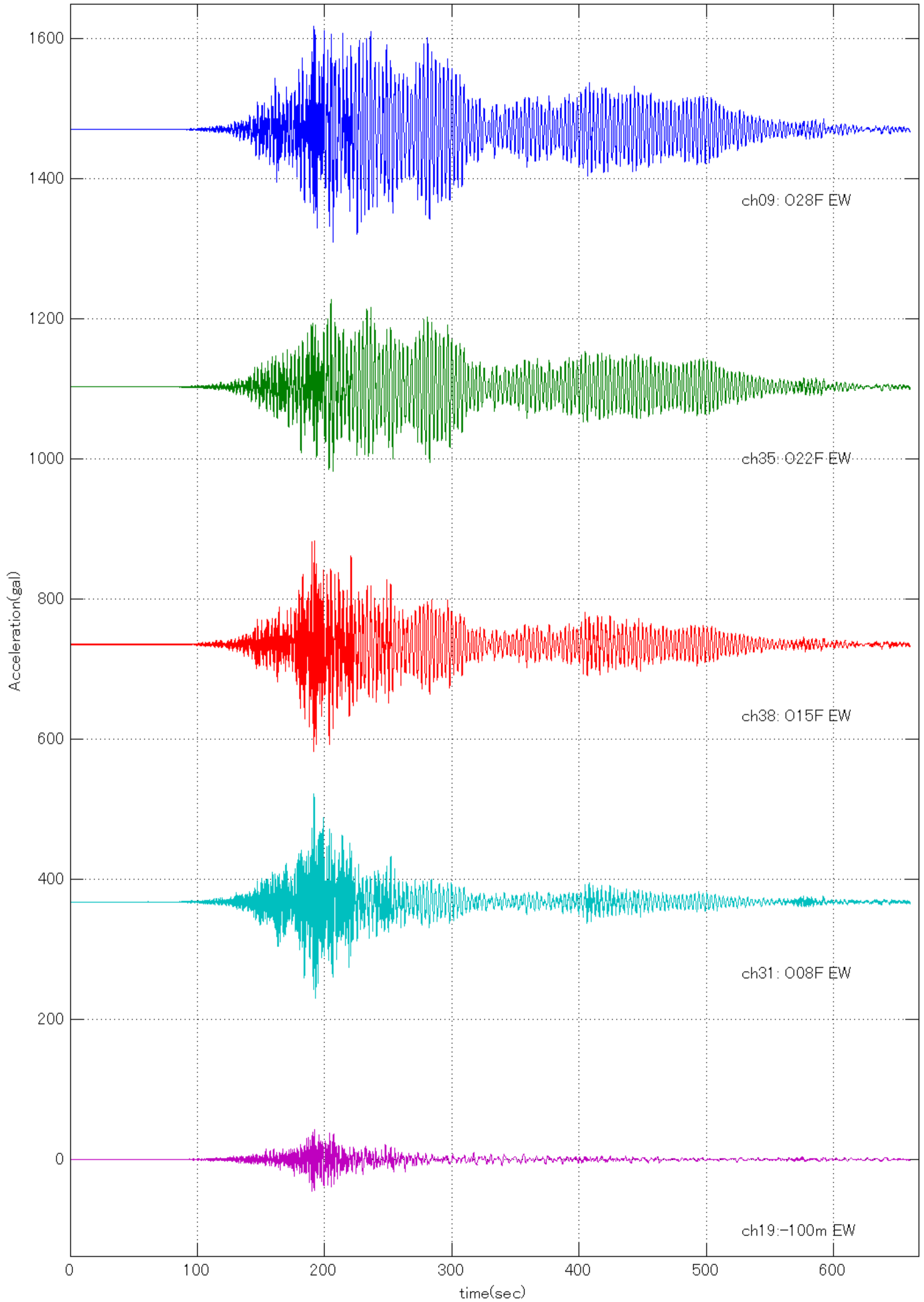
20110311144600 Quake (O28F EW: Max =147.0697 at 191.72 sec )
