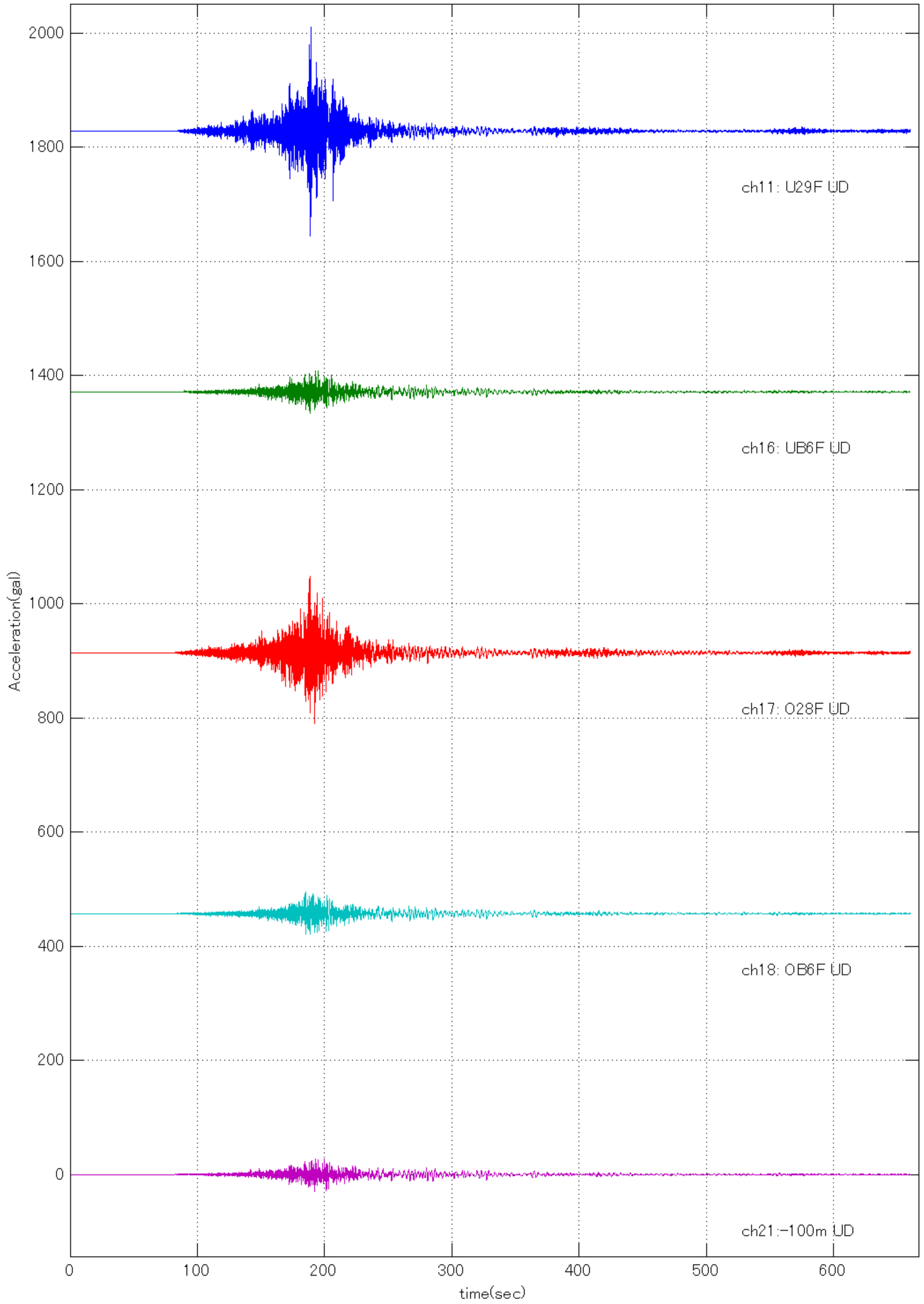
20110311144600 Quake (University 29F UD: Max =182.8072 at 189.18 sec )
