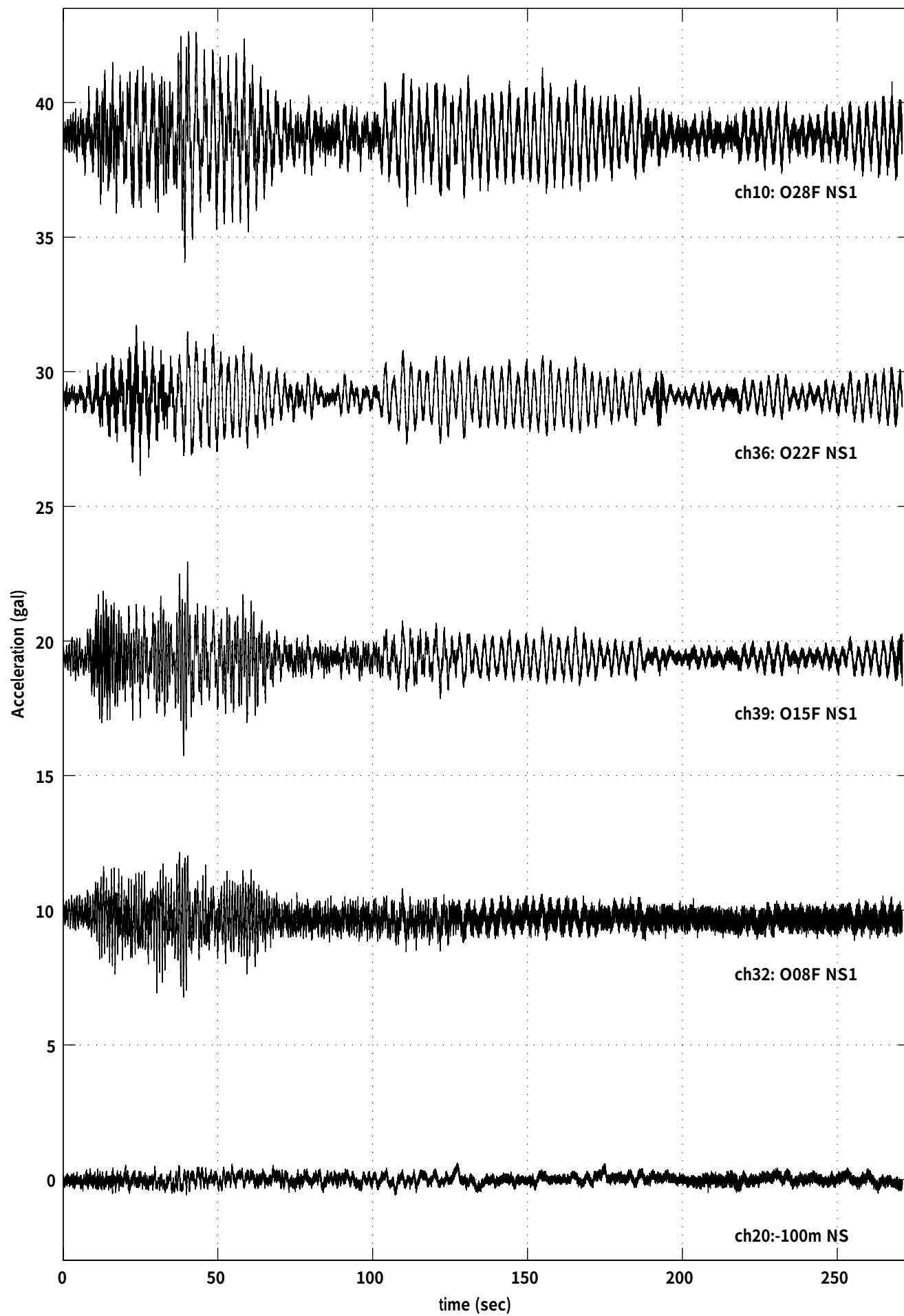
040907-0831 Quake (O28F NS1: Max =3.876 at 40.62 sec )
