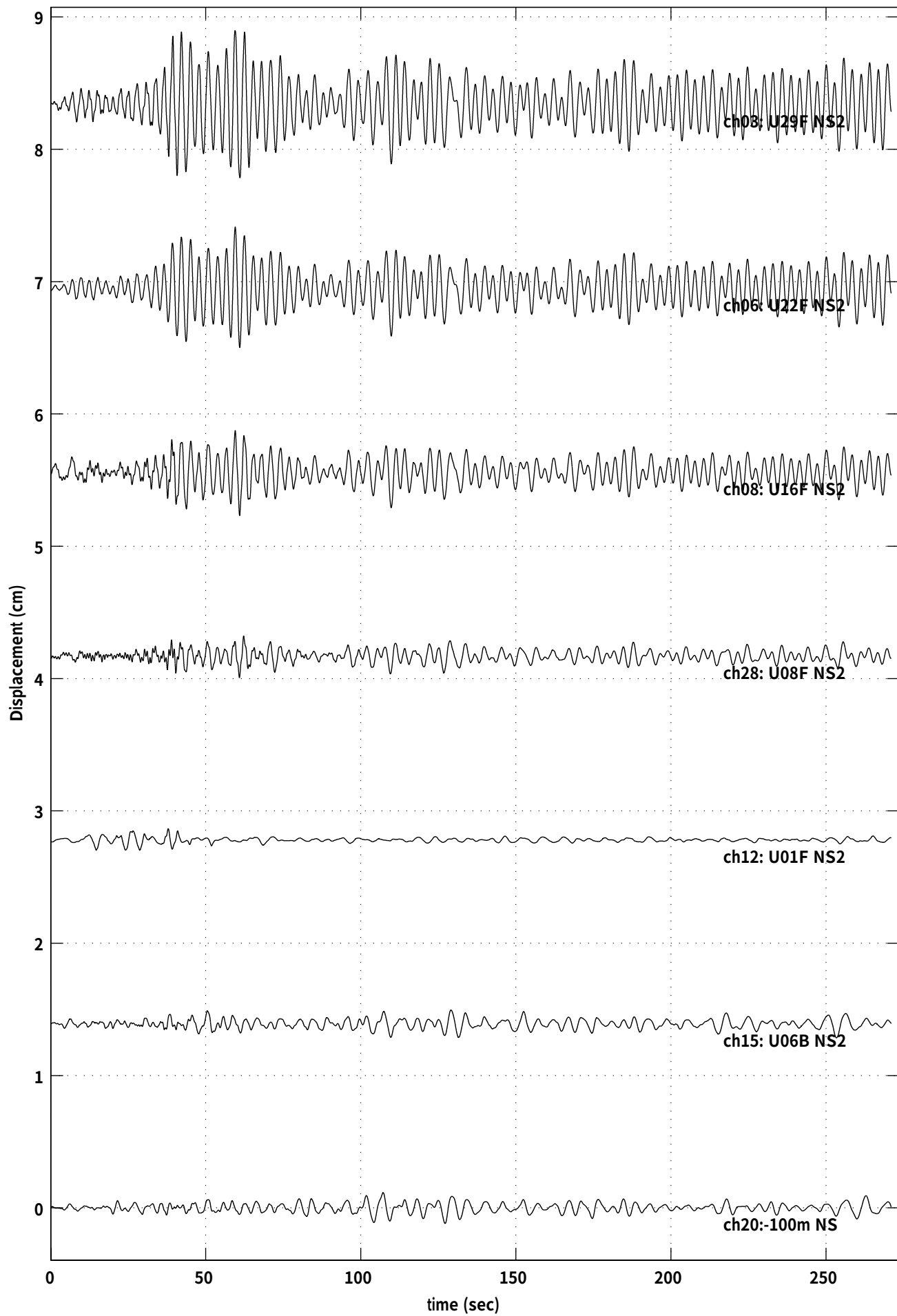
040907-0831 Quake (U29F NS2: Max =0.556 at 59.46 sec )
