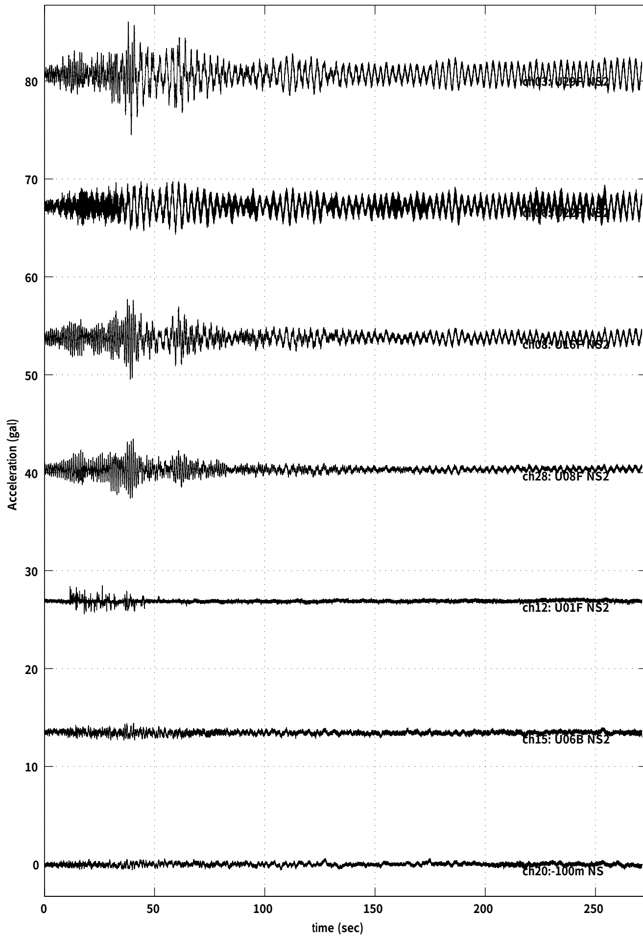
040907-0831 Quake (U29F NS2: Max =5.377 at 38.09 sec )
