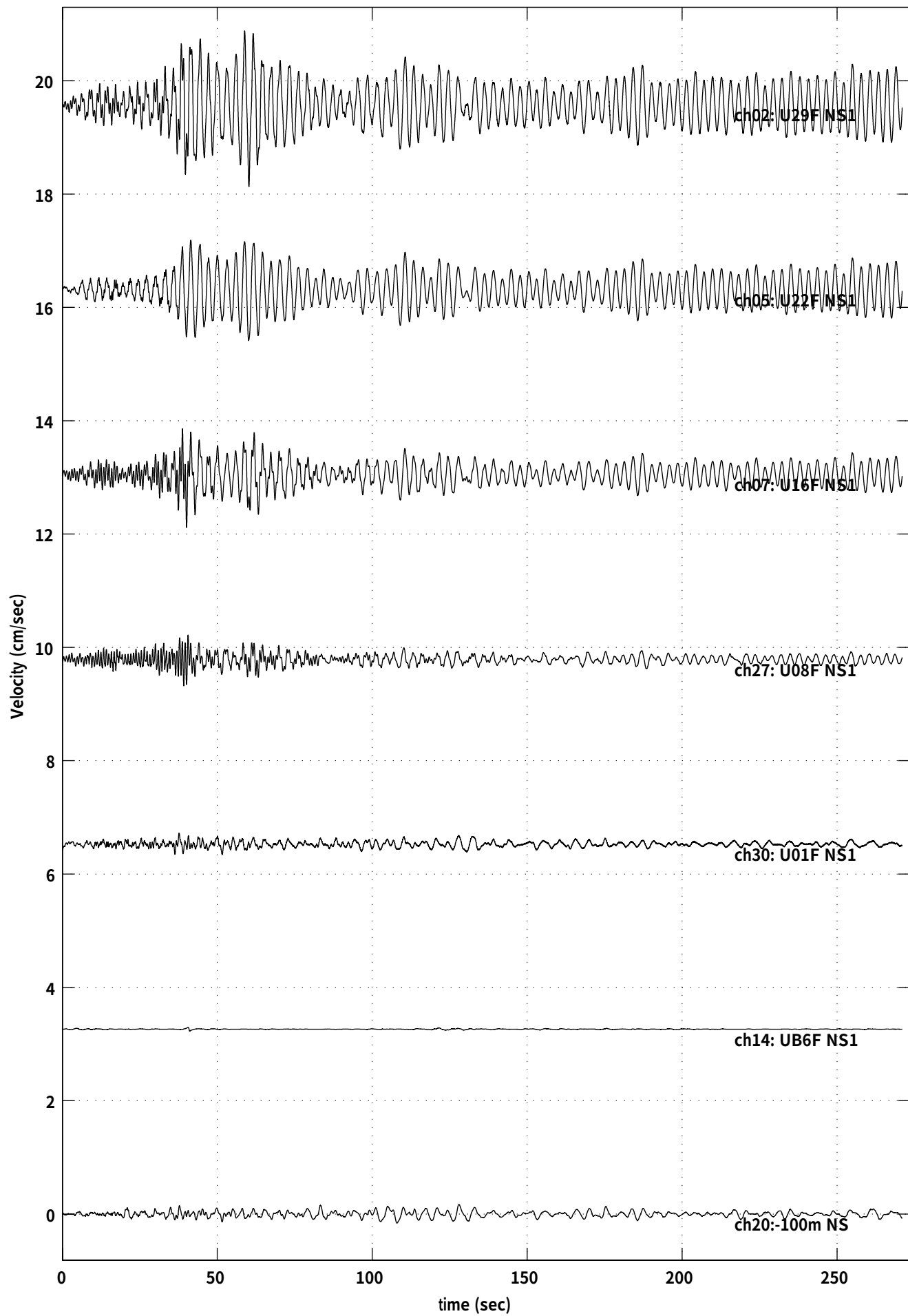
040907-0831 Quake (U29F NS1: Max =1.305 at 58.81 sec )
