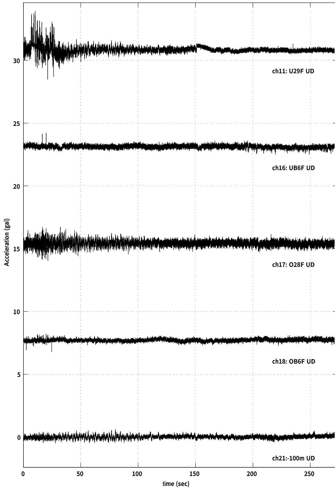
040907-0831 Quake (University 29F UD: Max =3.083 at 10.39 sec )
