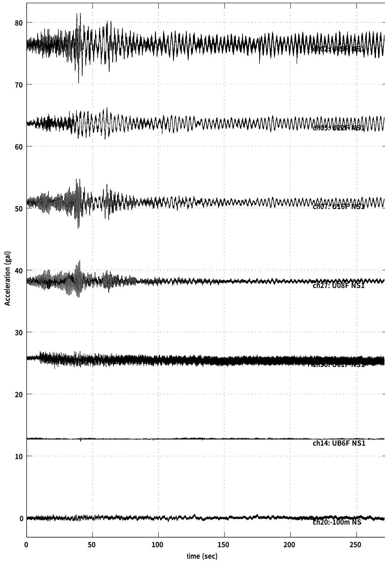
040907-0831 Quake (U29F NS1: Max =5.093 at 40.81 sec )
