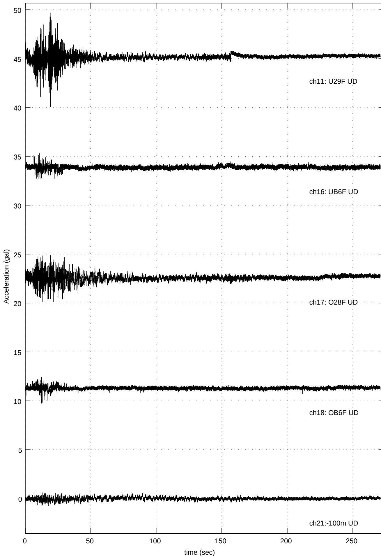
041025-0605 Quake (University 29F UD: Max =4.517 at 19.51 sec )
