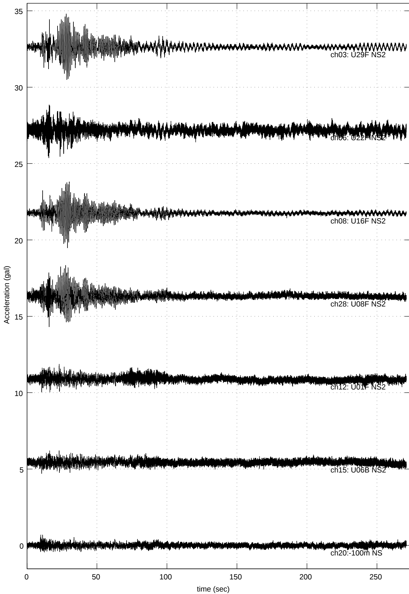
041025-0029 Quake (U29F NS2: Max =2.175 at 28.04 sec )
