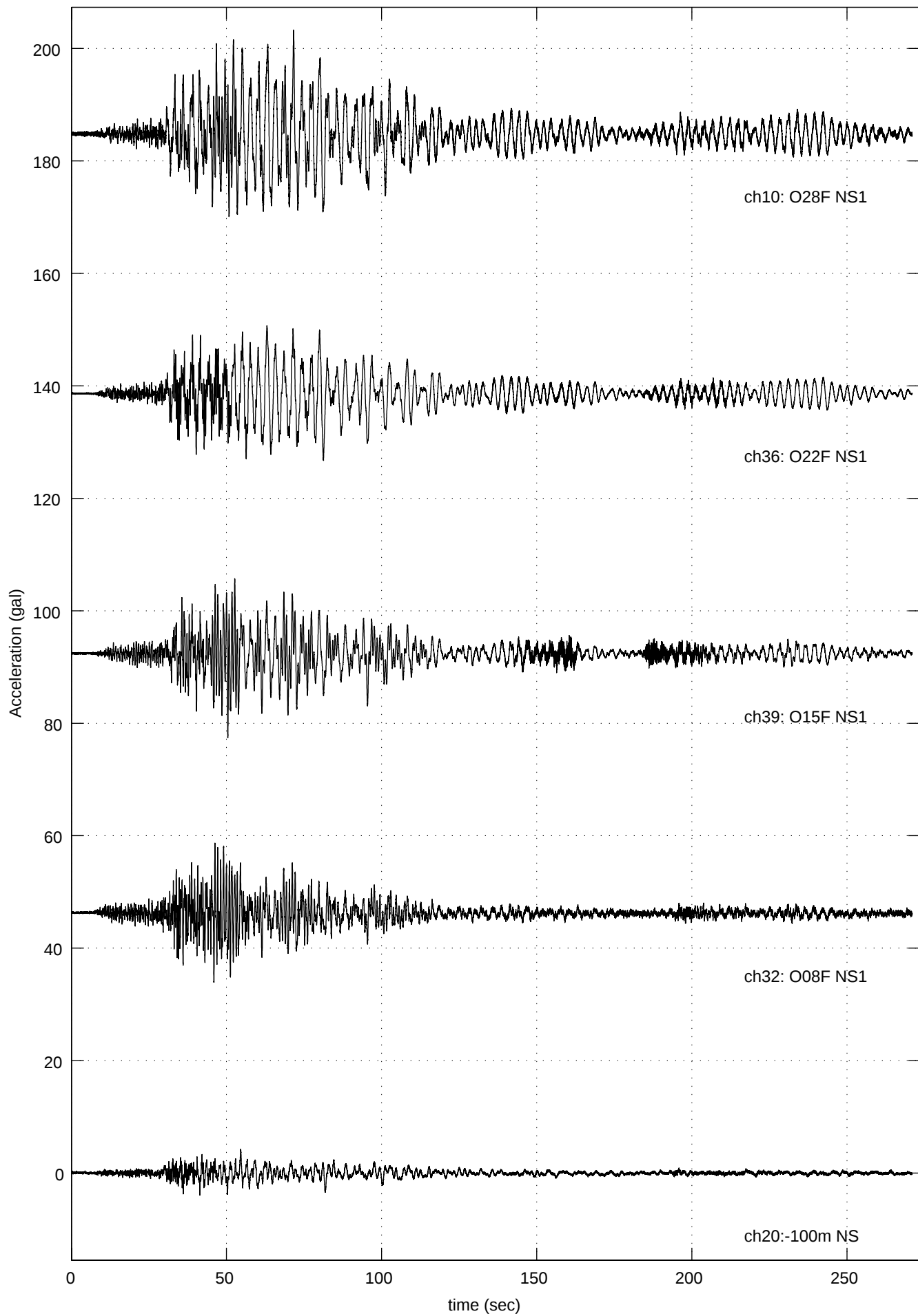
041023-1834 Quake (O28F NS1: Max =18.48 at 71.62 sec )
