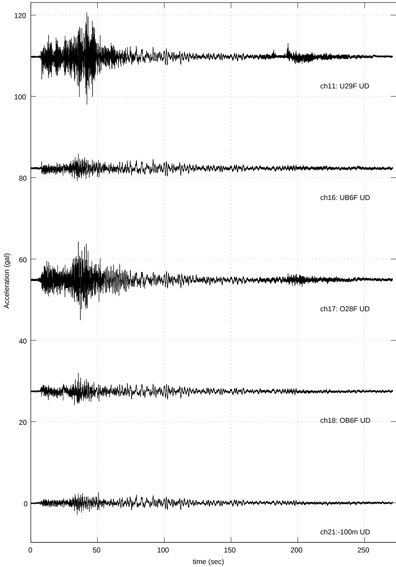
041023-1834 Quake (University 29F UD: Max =10.97 at 41.99 sec )
