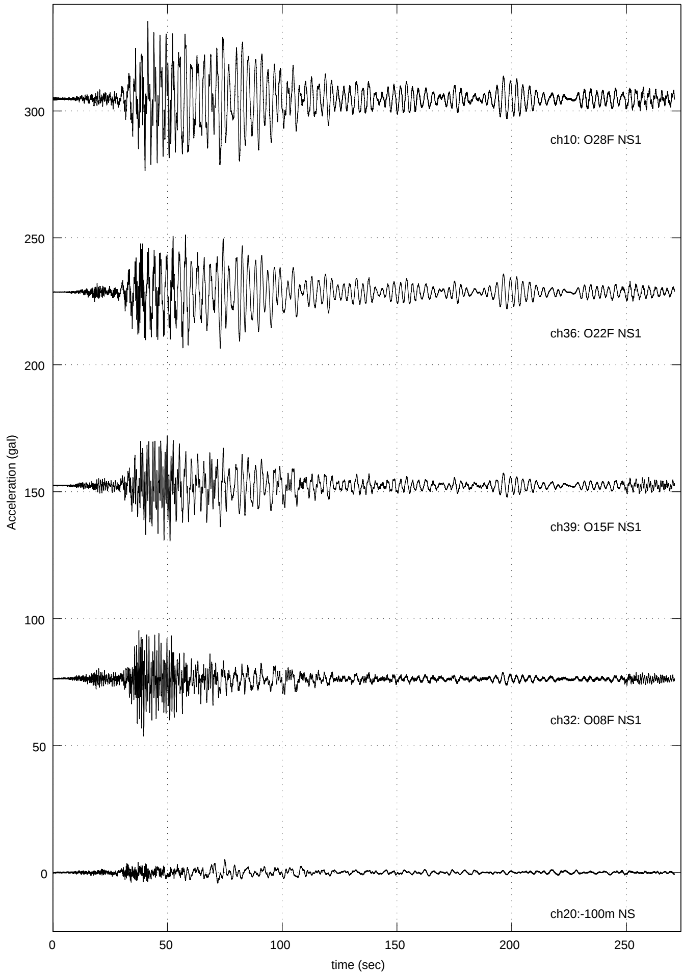
041023-1756 Quake (O28F NS1: Max =30.48 at 41.45 sec )
