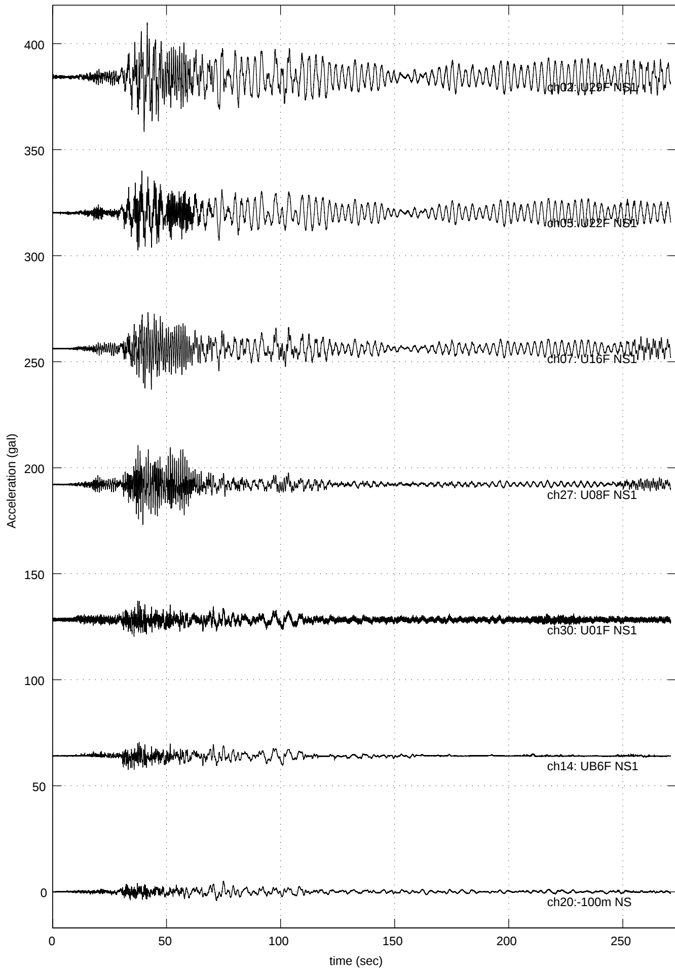
041023-1756 Quake (U29F NS1: Max =25.62 at 41.53 sec )
