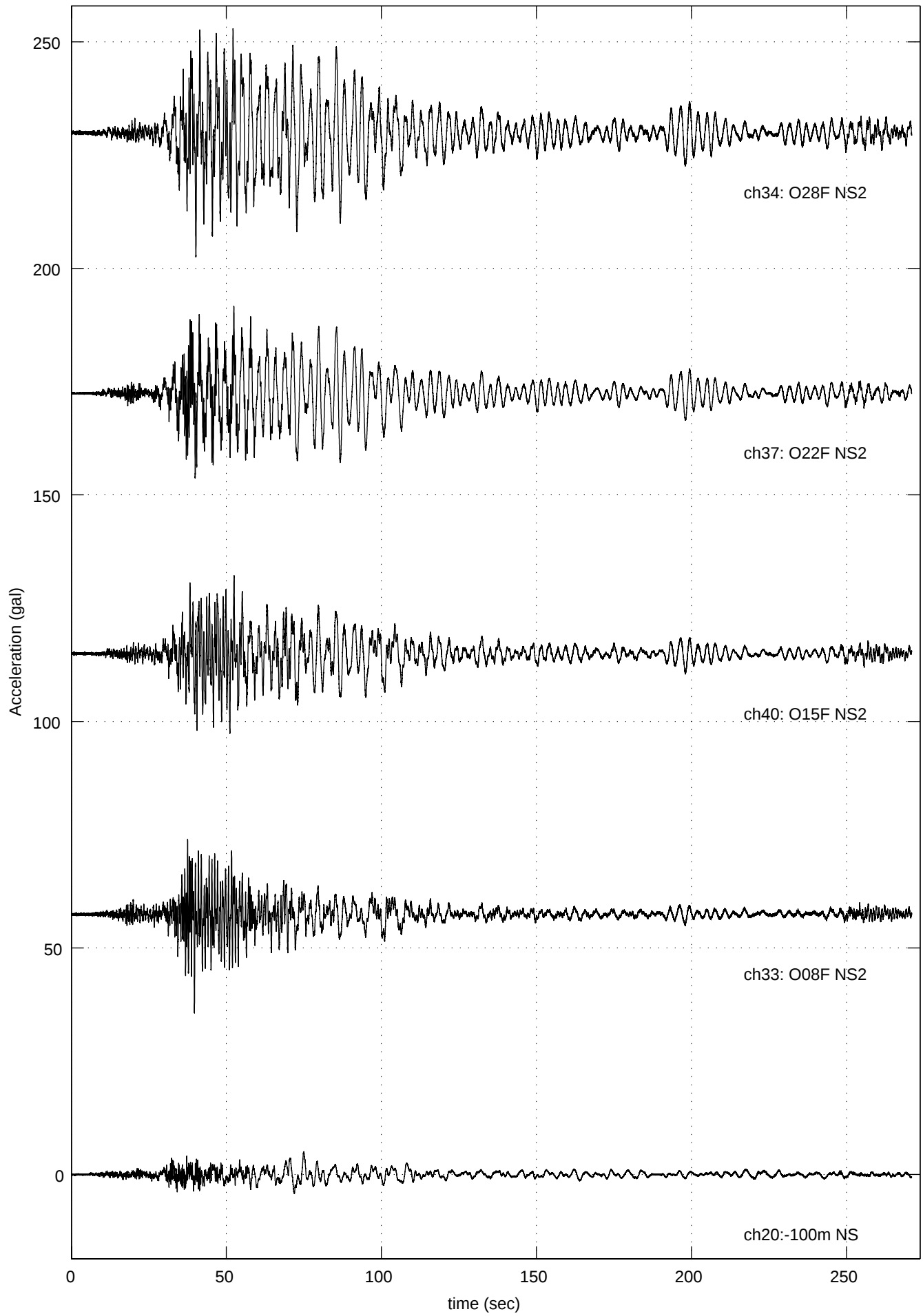
041023-1756 Quake (O28F NS2: Max =22.99 at 52.16 sec )
