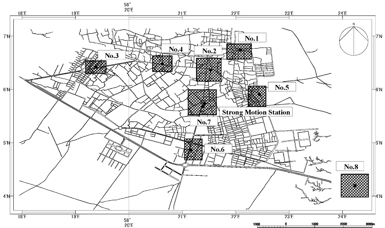
Fig. 4. Map of Bam city and the eight investigated areas (drawn from satellite image ; Kosugi, Lab., 2004).
