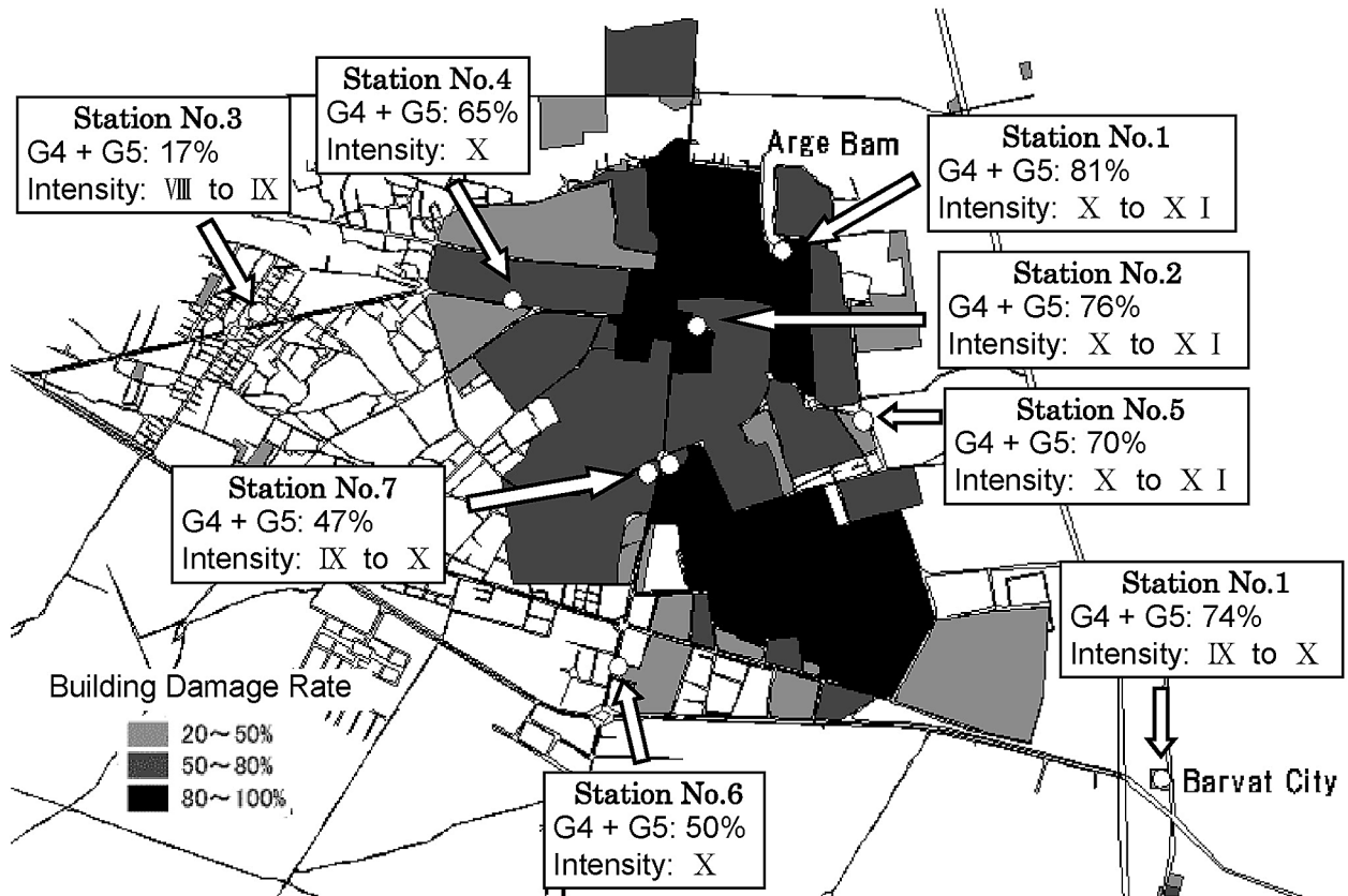
Fig. 7. Damage rates and estimated MSK intensities, together with damage map estimated from aerial photos independently 4) .
