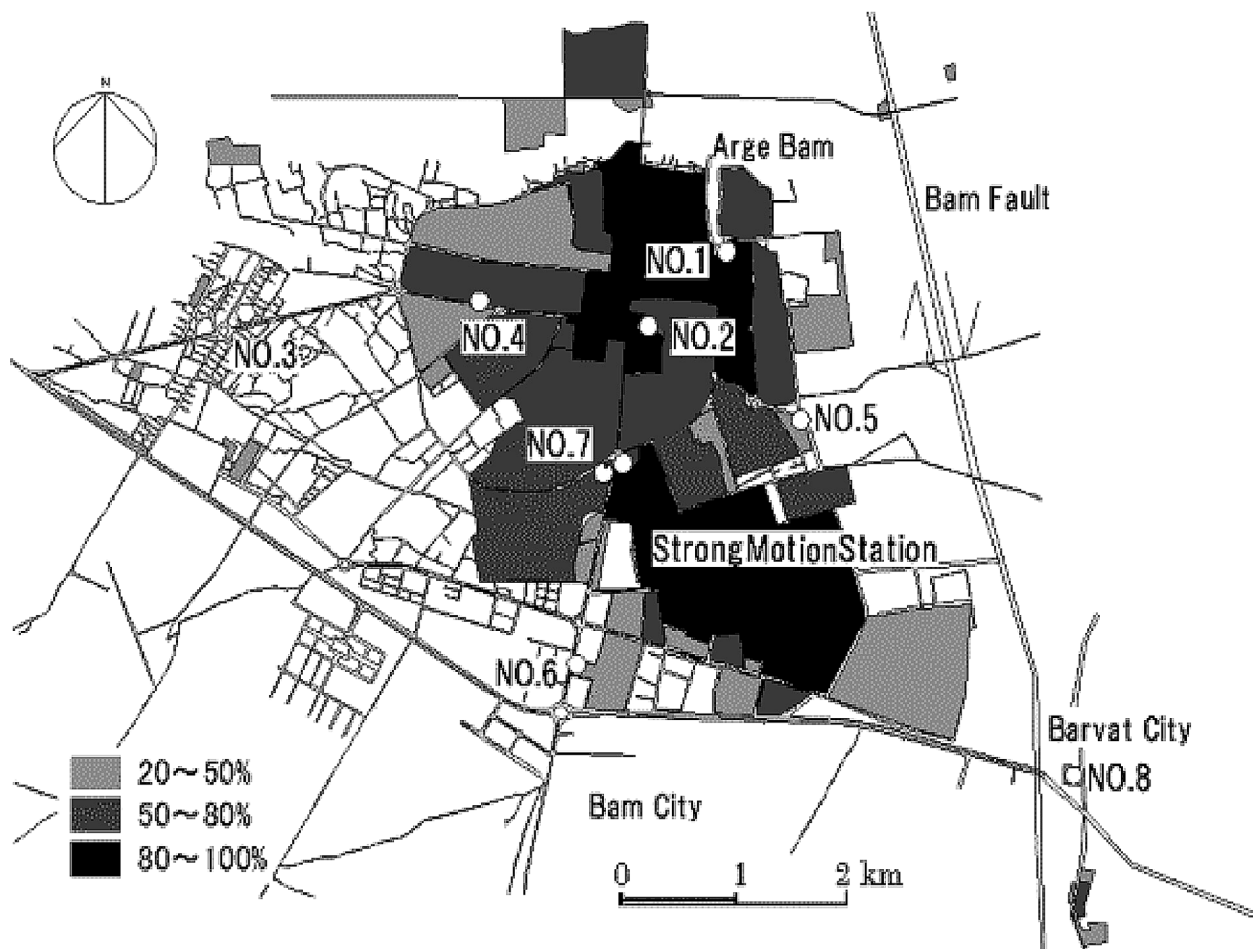
Fig. 2. Earthquake damage map of Bam and Baravat cities 4) and the strong motion and aftershock stations.
